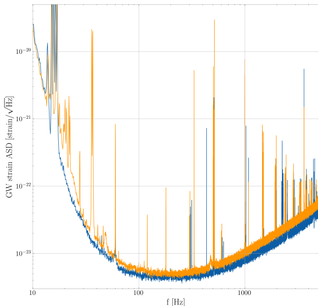
FIG. 1. Sensitivity plot GW strain amplitude spectral density (abbreviated as ASD on axis label) for LIGO-Hanford (orange) and LIGO-Livingston (blue) for a snapshot of data (10.0 minutes) from O3 (channel *:DCS-CALIB_STRAIN_C01_AR, see Ref. [47, 48]). The vertical axis plots the amplitude spectral density of the detector noise in units of \text{Hz}^{-1/2} , while the horizontal axis plots the observation frequency in units of Hz. The spectral line at 60 Hz is clearly visible as a spike rising three decades, along with multiple other instrumental lines at other frequencies.
