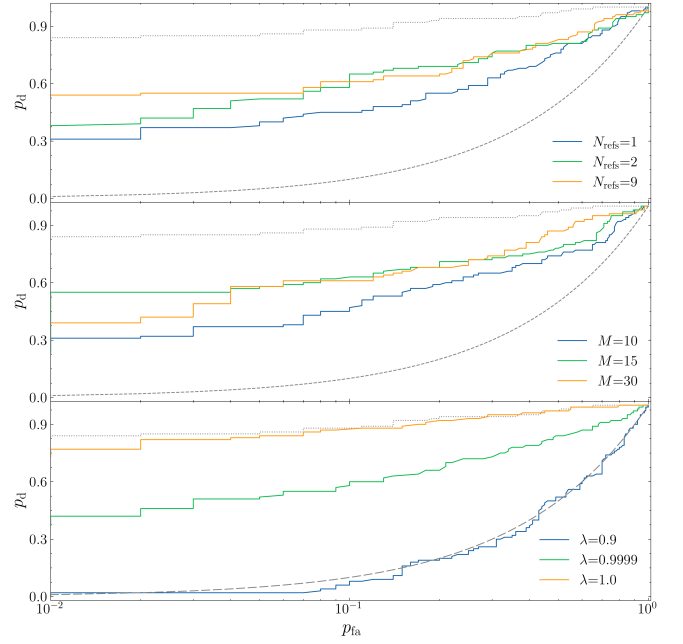
FIG. 9. Same as Figure 8 but for different ANC filter parameters. The top, middle and bottom panels display the ROC curves for different numbers of PEM reference channels N_{ref} , tap weights M , and forgetting factors \lambda respectively. All panels additionally include the ROC curve for a random classifier (i.e. the lower performance limit, grey dashed curve) and the zero interference ROC curve (i.e. the upper performance limit, grey dotted curve).
