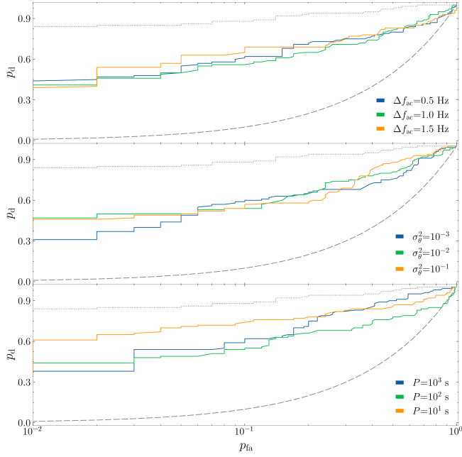
FIG. 8. Detection probability p_d as a function of false alarm probability p_{fa} (i.e. ROC curve) for HMM tracking of a CW signal ( h_0\sqrt{T_{obs}}/\sigma_n = 0.62 ) in conjunction with the ANC scheme, for different mains power interference parameters. The top, middle and bottom panels display different values of \Delta f_{ac} , \sigma_\Theta^2 , and P respectively. The grey dashed curve in all panels corresponds to the performance of a random classifier. The grey dotted curve in all panels is a performance upper limit, corresponding to the case where there is zero mains power interference. In all panels the curves overlap approximately, illustrating that the performance of the HMM and ANC scheme is insensitive to the mains power parameters. At p_{fa} = 0.05 , the mean p_d across the three curves is 0.52 (top panel), 0.48 (middle panel) and 0.58 (bottom panel).
