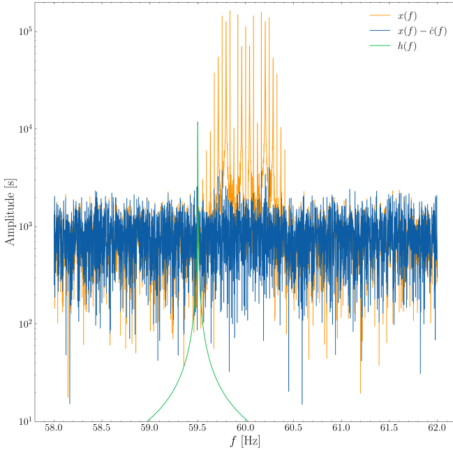
FIG. 6. Spectrum (i.e. modulus of the Fourier transform) of the data x(t) (orange curve), GW signal h(t) (green curve) and declustered output of the ANC filter x(t) - \hat{c}(t) (blue curve) for a system with parameters described in Table I. A peak in the blue curve at 59.5 Hz is partially obscured by the green curve. ANC suppresses by \approx 20 \text{ dB} \approx 40 \text{ dB} the orange spikes near 60 Hz, corresponding to mains power interference.
