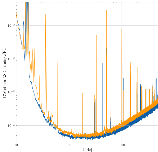
FIG. 1. Sensitivity-GW strain amplitude spectral density (ASD) plot for LIGO-Hanford (orange) and LIGO-Livingston (blue) for a snapshot of data (10.0 minutes) from O3 (channel *:DCS-CALIB_STRAIN_C01.AR, see Ref. [47, 48]). The vertical axis plots the amplitude spectral density of the detector noise in units of \text{Hz}^{-1/2} , while the horizontal axis plots the observation frequency in units of Hz. The spectral line at 60 Hz is clearly visible as a spike rising three decades, along with multiple other instrumental lines at other frequencies.
