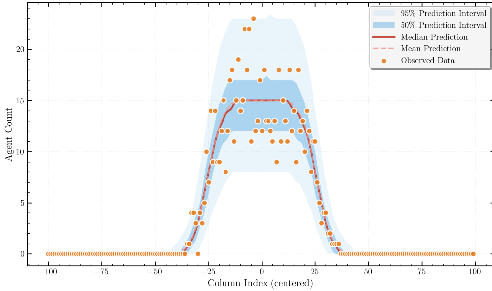
Figure 9: Posterior predictive checks from NPE using 1D column count data. The observed data (orange circles) is overlaid on predictions generated by simulating the model with parameters drawn from the inferred posterior distribution. The median (solid red line) and mean (dashed red line) of the predictions are shown, along with the 50% (dark blue) and 95% (light blue) prediction intervals. For visualization purposes, a Gaussian kernel has been applied to smooth the predictive distributions. An appropriate proportion of the observed data points lie within the 95% prediction interval, indicating that the calibrated model is consistent with the data.
