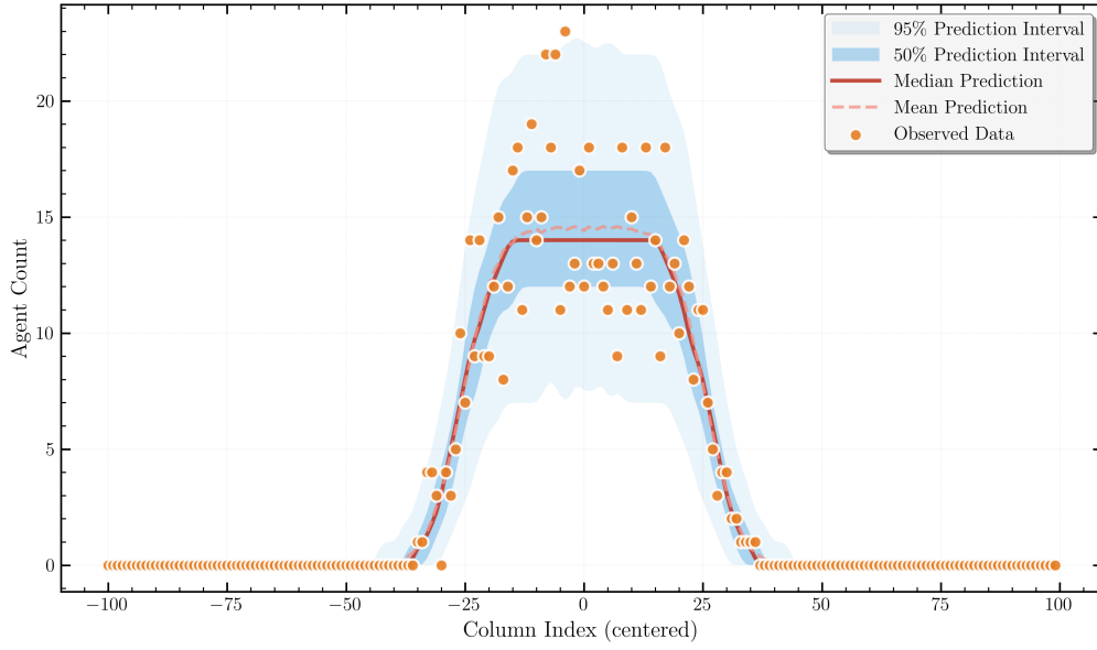
Figure 7: Posterior predictive check for the 2D spatial data model. The format is identical to Figure 5. The predictions are well-calibrated and consistent with the observed data.
