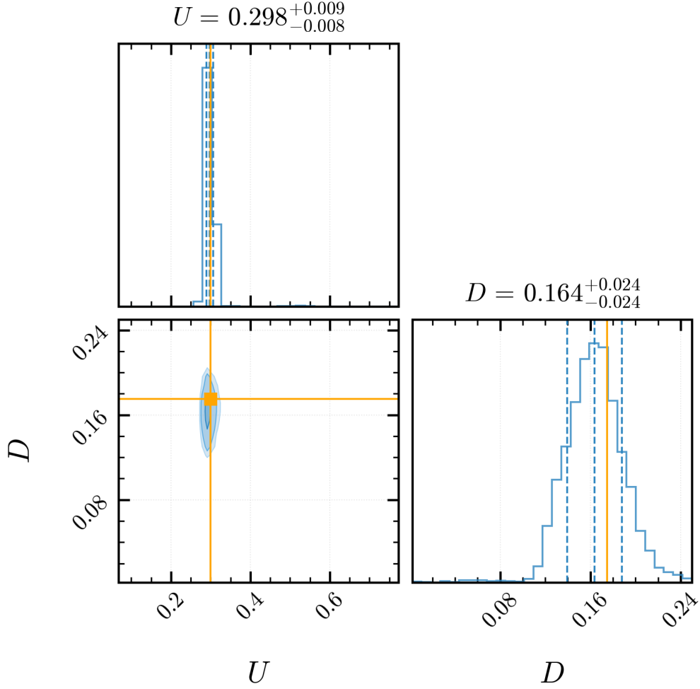
Figure 4: Posterior distribution from NPE using 1D column count data. The figure is arranged as described in Figure 2. The true parameter values (orange cross) are contained within the 68% credible interval
