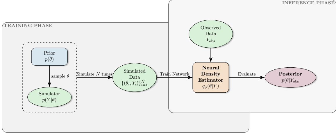
Figure 3: Schematic overview of the NPE workflow. The training phase (left) involves sampling parameters from the prior, generating simulated data, and training a neural density estimator on the resulting parameter-data pairs. The inference phase (right) uses the trained network to instantly evaluate the posterior for new observations without additional simulations.
