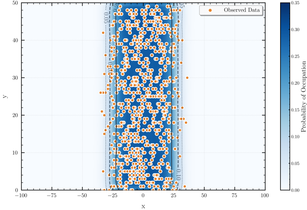
Figure 7: Posterior predictive check for the 2D spatial data model, showing the full observed data points (orange) overlaid on the predicted occupancy probability from the NPE model (blue heatmap). The grey contours delineate iso-probability curves at probability levels of 0.05, 0.10, and 0.20 (dotted, dashed, solid, respectively)
