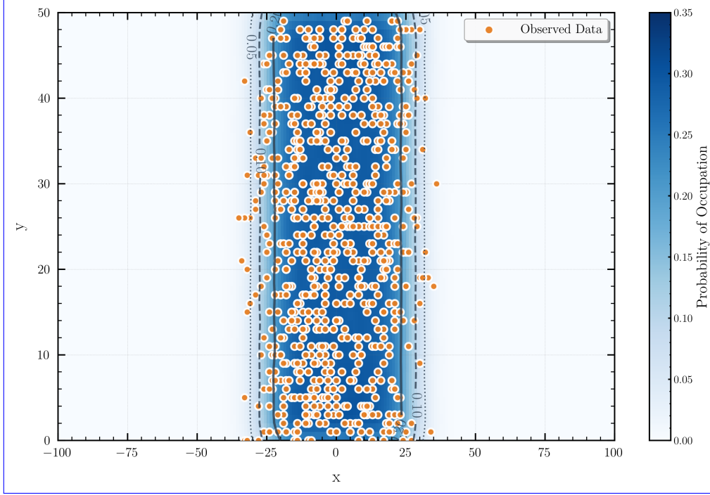
Figure 7: Posterior predictive check for the 2D spatial data model, showing the full observed data points (orange) overlaid on the predicted occupancy probability from the NPE model (blue heatmap). The grey contours delineate iso-probability curves at probability levels of 0.05, 0.10, and 0.20 (dotted, dashed, solid, respectively)
