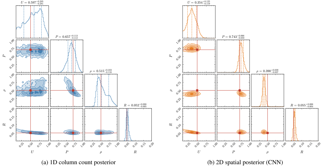
Figure 7: Posterior distributions for Model C (bias + proliferation) with true values U = 0.5 , P = 0.7 , \rho = 0.5 , R = 0.05 . Despite the four-parameter space and absence of a tractable likelihood, NPE recovers all parameters with well-calibrated uncertainty estimates.
