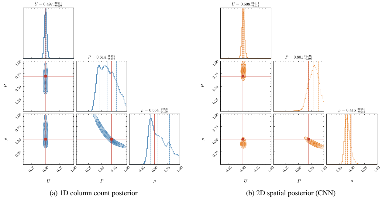
Figure 5: Posterior distributions for Model A (directional bias) with true values U = 0.5 , P = 0.7 , \rho = 0.5 . Both representations recover U precisely but exhibit a strong P - \rho anti-correlation reflecting the drift velocity degeneracy v = P\rho/2 .
