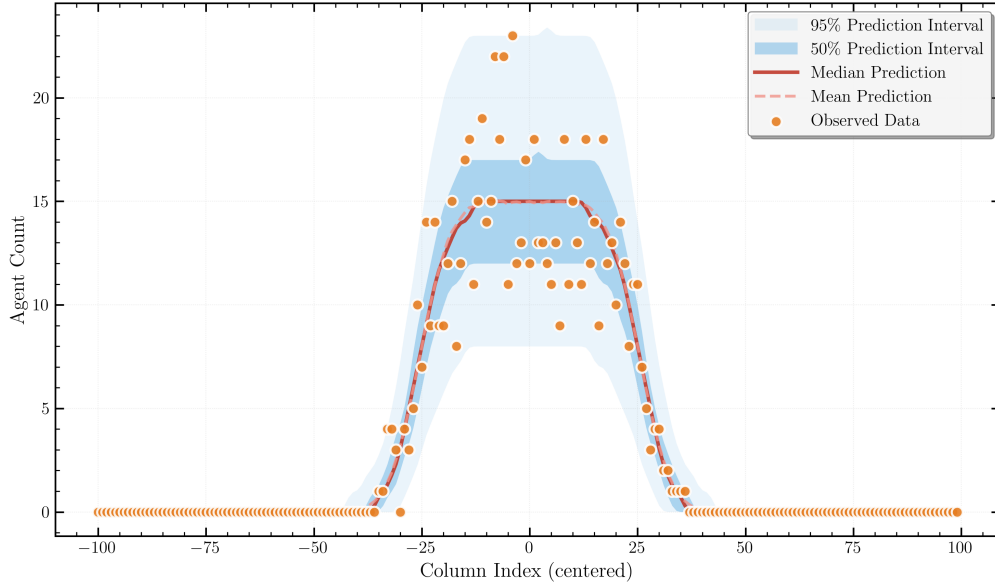
Figure 9: Posterior predictive checks from NPE using 1D column count data. The observed data (orange circles) is overlaid on predictions generated by simulating the model with parameters drawn from the inferred posterior distribution. The median (solid red line) and mean (dashed red line) of the predictions are shown, along with the 50% (dark blue) and 95% (light blue) prediction intervals. For visualization purposes, a Gaussian kernel has been applied to smooth the predictive distributions. An appropriate proportion of the observed data points lie within the 95% prediction interval, indicating that the calibrated model is consistent with the data.
