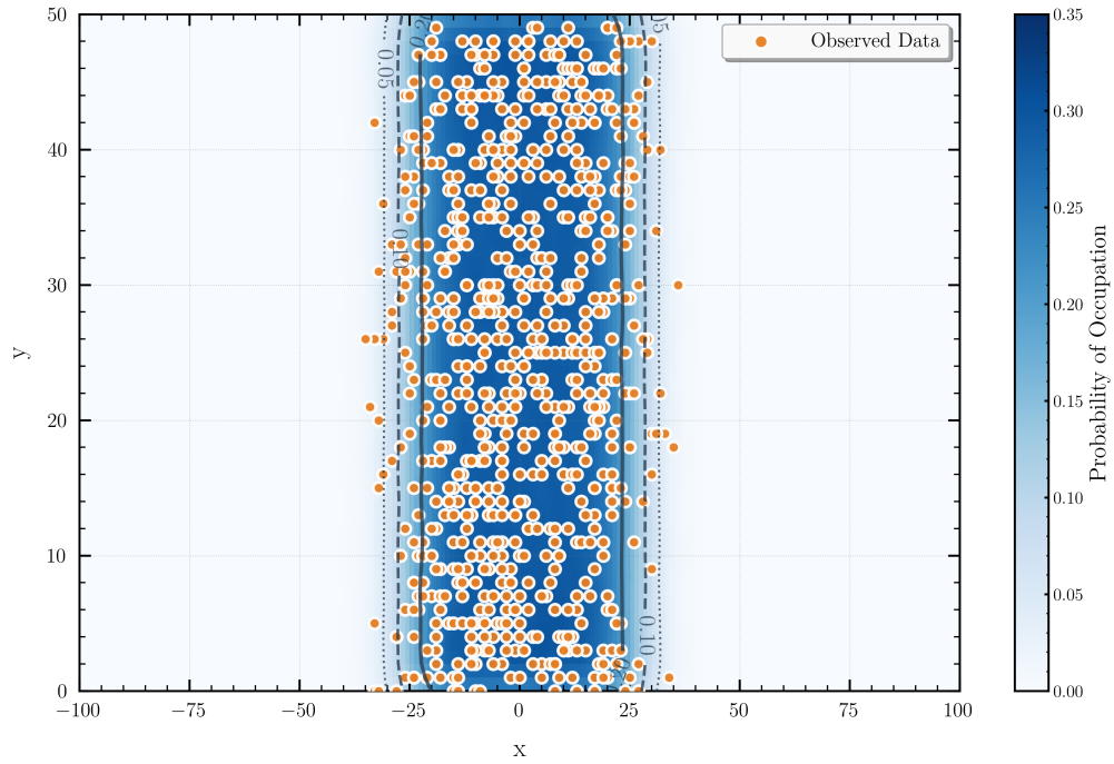
Figure 10: Posterior predictive check for the 2D spatial data model, showing the full observed data points (orange) overlaid on the predicted occupancy probability from the NPE model (blue heat-map). The grey contours delineate iso-probability curves at probability levels of 0.05, 0.10, and 0.20 (dotted, dashed, solid, respectively).
