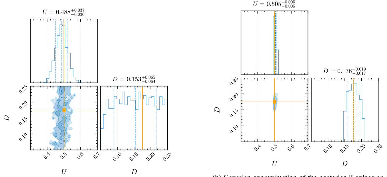
(b) Gaussian approximation of the posterior (Laplace approximation) via MLE on a deterministic surrogate model. This approach is computationally efficient but conditional on the surrogate's fidelity.
