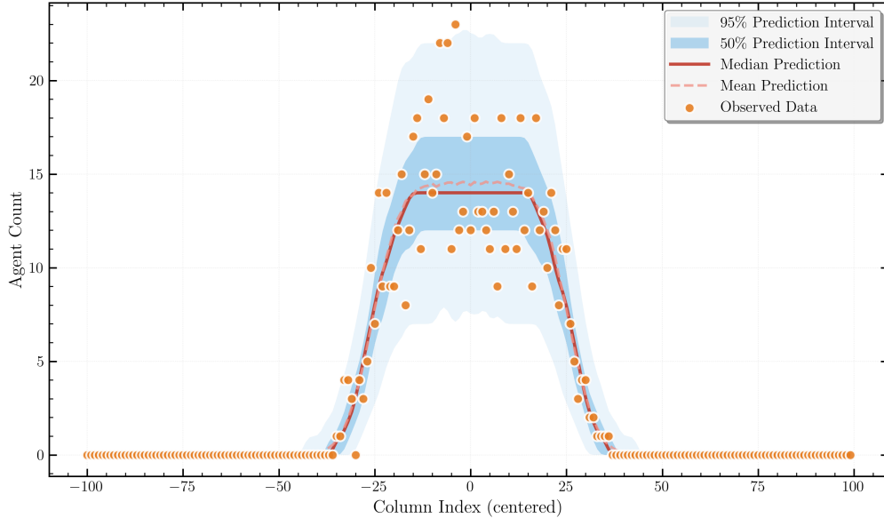
Figure 5: Posterior predictive check for the 2D spatial data model. The format is identical to Figure 3. The predictions are well-calibrated and consistent with the observed data.
