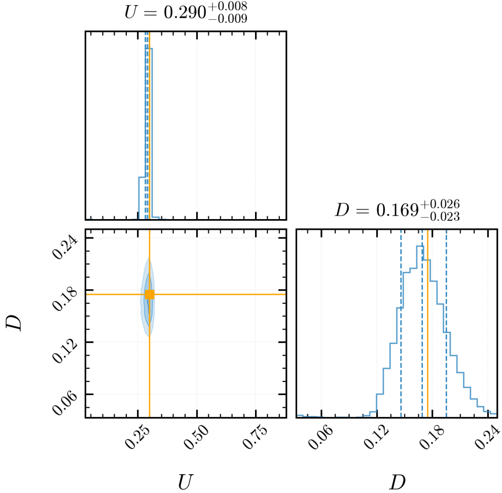
Figure 4: As Figure 2, for posteriors generated from the NPE with CNN embedding networks, using full 2D spatial data.
