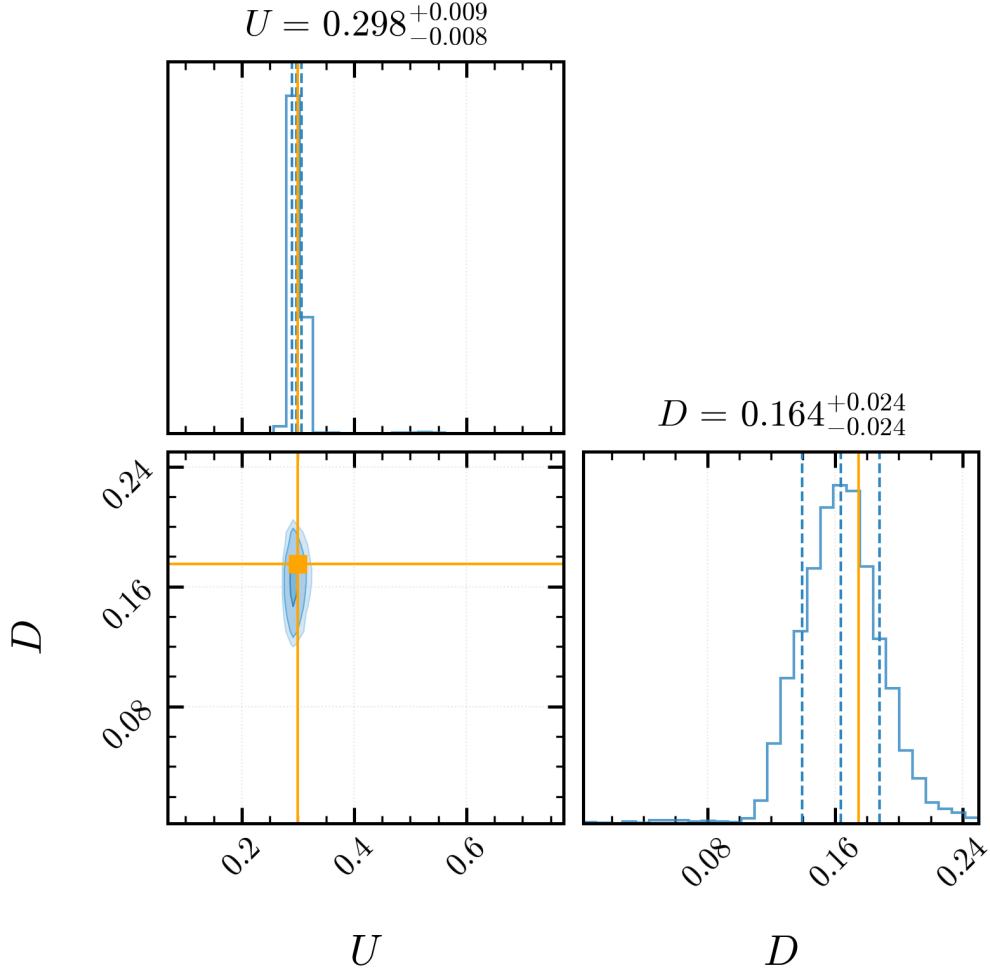
Figure 2: Posterior distribution from NPE using 1D column count data. The contours show 68% and 95% credible regions, with the true parameter values (orange cross) falling well within the high-probability region.
