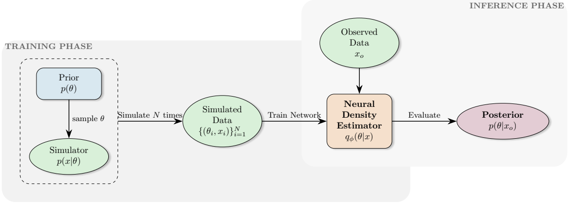
Figure 3: Schematic overview of the Neural Posterior Estimation (NPE) workflow. The training phase (left) involves sampling parameters from the prior, generating simulated data, and training a neural density estimator on the resulting parameter-data pairs. The inference phase (right) uses the trained network to instantly evaluate the posterior for new observations without additional simulations.
