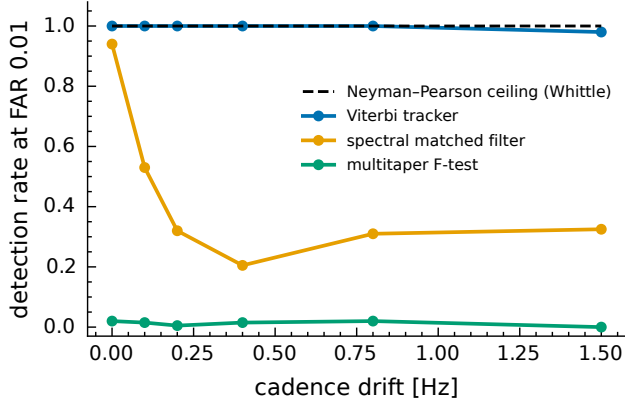
Figure 3. Detection rate at empirical false-alarm rate 10^{-2} against the inference null, versus cadence drift ( n = 200 per class, 300 s traces). The Viterbi tracker holds the Whittle Neyman-Pearson ceiling across the wander axis; the spectral matched filter collapses once the line moves and the multitaper F-test has no usable power. The full bake-off, including the order-tracked statistics and structural-confuser negatives, is in Appendix C. Reproduced by scripts/plot_drift_ceiling.py .
