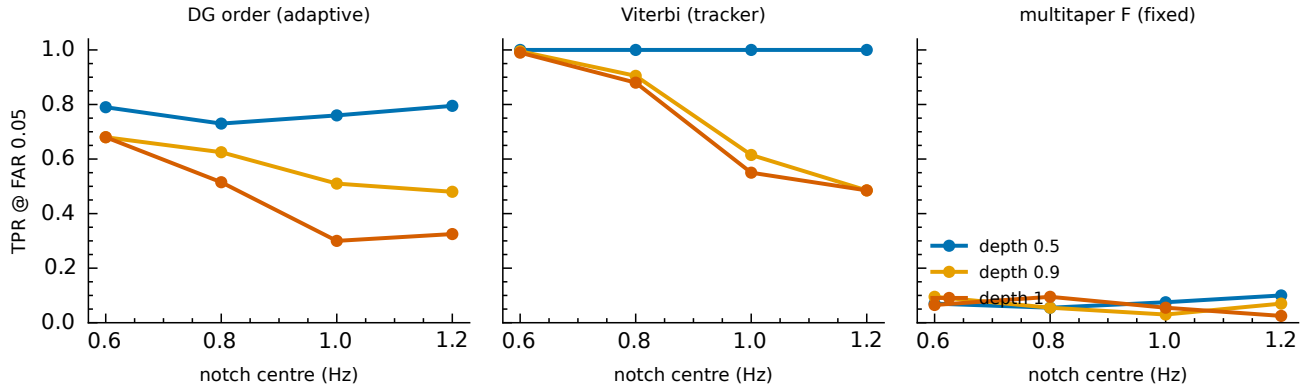
Figure 14. Transfer-function notch sub-sweep at 20 Hz sampling: tracker power versus notch centre frequency and depth. Only a deep notch placed at the cadence centre (1.0–1.2 Hz) materially degrades detection, and it halves rather than erases it.
