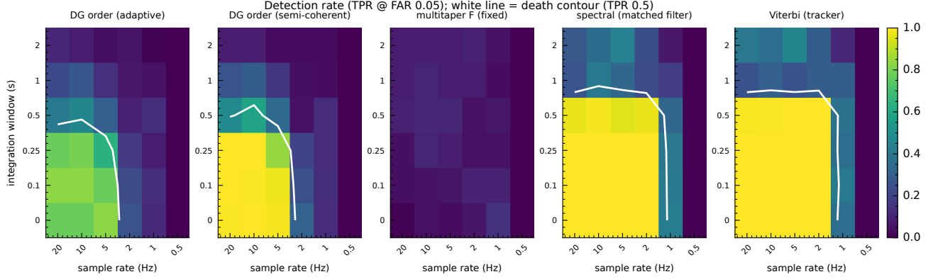
Figure 13. Minimum meter specification: detector power at nominal false-alarm rate 0.05 over sample rate \times integration window, one panel per detector, honest training against the hard inference null. The live region is sample rate \geq 2 Hz and integration window \leq 0.5 s; below either edge the tracking class collapses toward chance.
