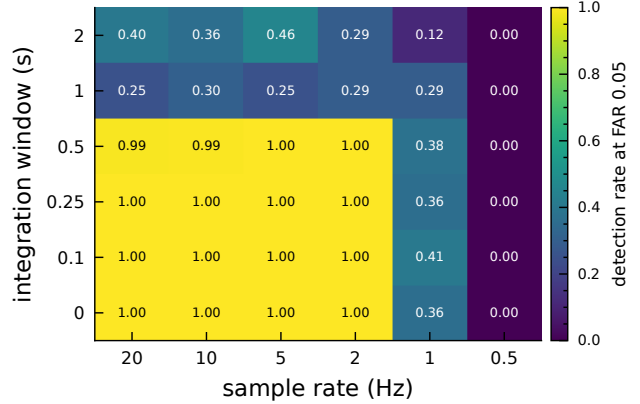
Figure 4. Minimum meter specification: Viterbi detection rate at nominal false-alarm rate 0.05 over sample rate \times integration window, honest training against the inference null ( n = 200 per class). The live region is sample rate \geq 2 Hz and integration window \leq 0.5 s. The per-detector grid is in Appendix E. Reproduced by scripts/plot_st2_meter_boundary.py .
