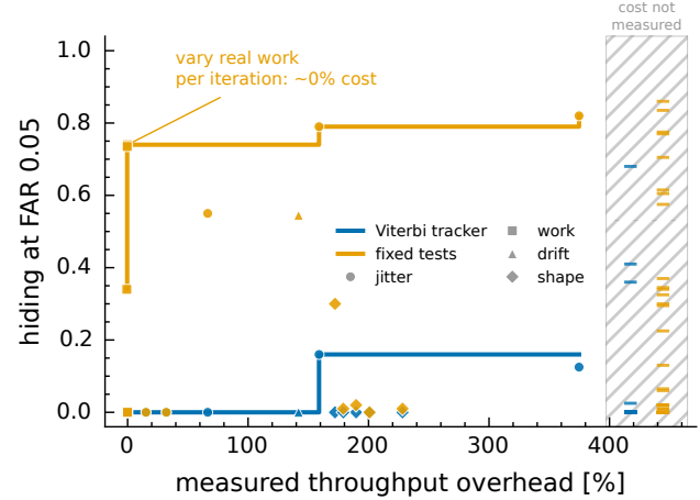
Figure 5. Cost of hiding. Measured throughput overhead against hiding (1 – detection rate at false-alarm rate 0.05) for the four attack families with a hardware cost anchor, with the Pareto staircase — the best hiding available at or below a given cost — against the fixed tests (orange; the better of the matched filter and multitaper F-test per cell) and the Viterbi tracker (blue). Varying real work per iteration hides \sim 0.74 from the fixed tests at no measurable cost; against the tracker no anchored attack hides more than 0.16. Cells without a cost anchor are shown as ticks in the hatched strip, among them work-variation level 0.7, where the tracker begins to fail. Reproduced by scripts/plot_money_pareto.py .
