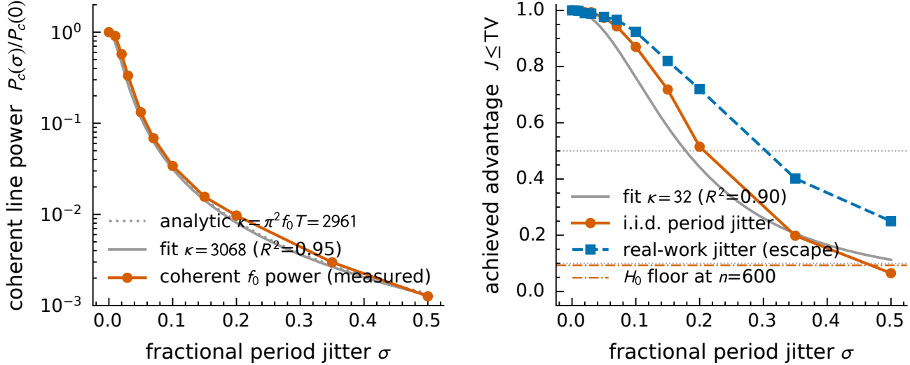
Figure 17. Numerical check on the covertness cost bound, through the full generator and meter ( n = 600 per class). Left: coherent power at the nominal cadence against jitter scale. The fitted and the parameter-free analytic rolloffs of Equations (14) and (16) are indistinguishable at this scale; the fitted constant agrees with the parameter-free prediction at the ten-percent level (see the numerical check). Right: the advantage attained by the fixed-bin threshold test, J \leq TV , for idle-padded period jitter and for the near-free work-varying attack; dotted lines mark \varepsilon \in \{0.1, 0.5\} , whose crossings give \sigma^*(\varepsilon) (the \varepsilon = 0.1 crossing lies beyond the swept range and is reached by extrapolation). The dash-dotted line is the H_0 fluctuation of the estimator: the \sigma = 0.5 point falls below it and is excluded from the advantage fit shown here (it is retained in the coherent-power fit on the left, which has no sampling floor of its own). For \sigma \geq 0.05 the work-varying attack is the more detectable of the two at matched distortion, the comparison the cost-of-hiding assumption appeals to; below that the two are indistinguishable within sampling error. Both arms set the period-jitter scale explicitly, so the distortion really is matched. The verifier here is fixed at the known cadence, not the order tracker of Section 4.
