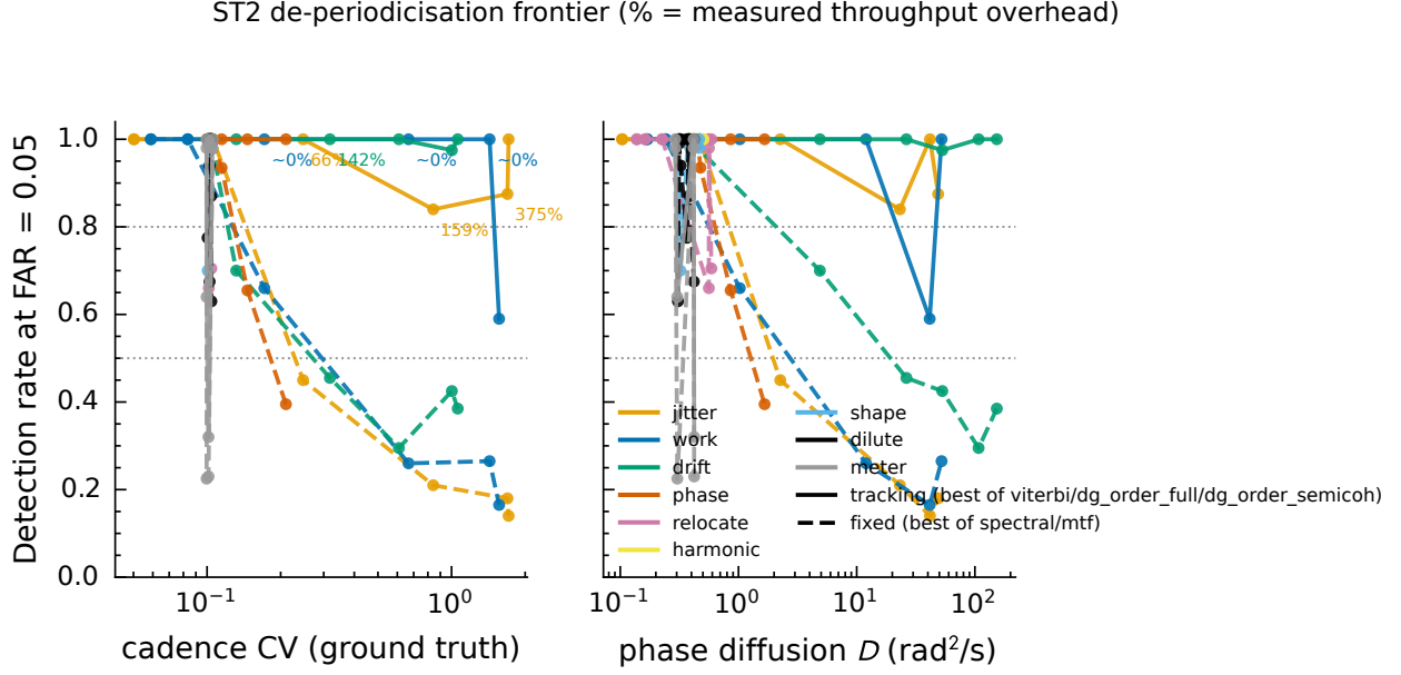
Figure 3: The de-periodicisation frontier: physical de-periodicisation (cadence coefficient of variation) against best tracking and best fixed detector power at nominal false-alarm rate 0.05, over all attack families. The near-vertical drop of the fixed class at the variable-real-work family, at essentially zero throughput cost, while the tracking class holds, is the scope boundary; costlier families (idle jitter, drift, shaping) sit at high throughput overhead without erasing the tracked line.
