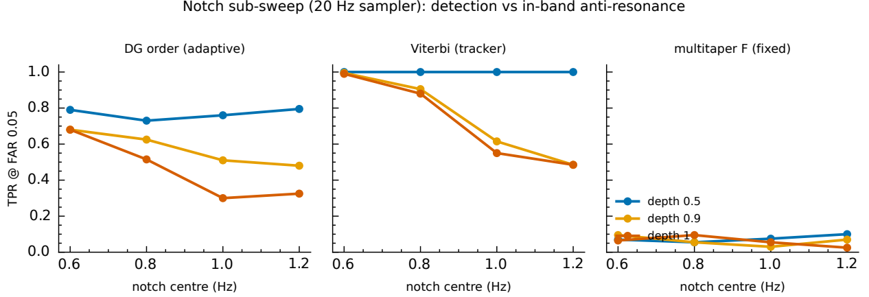
Figure 7: Transfer-function notch sub-sweep at 20 Hz sampling: tracker power versus notch centre frequency and depth. Only a deep notch placed at the cadence centre (1.0–1.2 Hz) materially degrades detection, and it halves rather than erases it.
