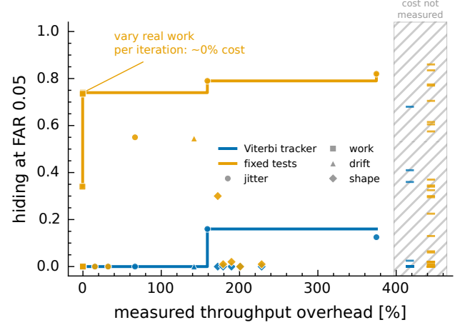
Figure 7. Cost of hiding. Measured throughput overhead against hiding (1– detection rate at false-alarm rate 0.05) for the four adversarial strategies with a hardware cost anchor, with the Pareto staircase — the best hiding available at or below a given cost — against the fixed tests (orange; the better of the matched filter and multitaper F-test per cell) and the Viterbi tracker (blue). Varying real work per iteration hides \sim 0.74 from the fixed tests at no measurable cost; against the tracker no anchored attack hides more than 0.16. Cells without a cost anchor are shown as ticks in the hatched strip, among them work-variation level 0.7, where the tracker begins to fail. Reproduced by scripts/plot_money_pareto.py .
