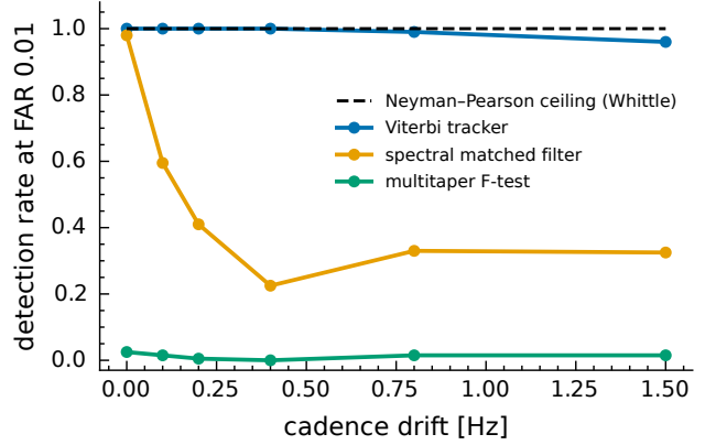
Figure 5. Detection rate at empirical false-alarm rate 10^{-2} against the null aggregate, versus cadence drift of the dominant training run ( n = 200 per class, 300 s traces, shares 9 : 0.5 : 0.5). The Viterbi tracker holds the Whittle Neyman–Pearson ceiling across the wander axis; the spectral matched filter collapses once the line moves and the multitaper F-test has no usable power. The full bake-off, including the order-tracked statistics and structural-confuser negatives, is in Appendix C. Reproduced by scripts/plot_drift_ceiling.py --scenario aggregate .
