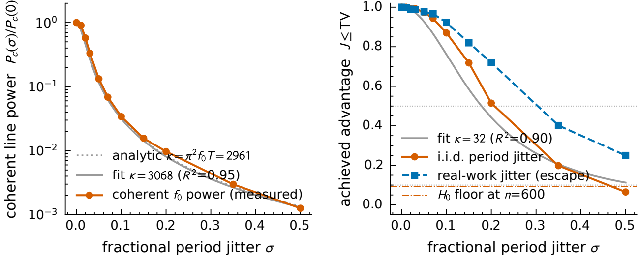
Figure 19. Numerical check on the covertness cost bound, through the full generator and meter ( n = 600 per class). Left: coherent power at the nominal cadence against jitter scale. The fitted and the parameter-free analytic rollofts of Equations (21) and (23) are indistinguishable at this scale; the fitted constant agrees with the parameter-free prediction at the ten-percent level (see the numerical check). Right: the advantage attained by the fixed-bin threshold test, J \leq TV , for idle-padded period jitter and for the near-free work-varying attack; dotted lines mark \varepsilon \in \{0.1, 0.5\} , whose crossings give \sigma^*(\varepsilon) (the \varepsilon = 0.1 crossing lies beyond the swept range and is reached by extrapolation). The dash-dotted line is the H_0 fluctuation of the estimator: the \sigma = 0.5 point falls below it and is excluded from the advantage fit shown here (it is retained in the coherent-power fit on the left, which has no sampling floor of its own). For \sigma \geq 0.05 the work-varying attack is the more detectable of the two at matched distortion, the comparison the cost-of-hiding assumption appeals to; below that the two are indistinguishable within sampling error. Both arms set the period-jitter scale explicitly, so the distortion really is matched. The verifier here is fixed at the known cadence, not the order tracker of Section 4.
