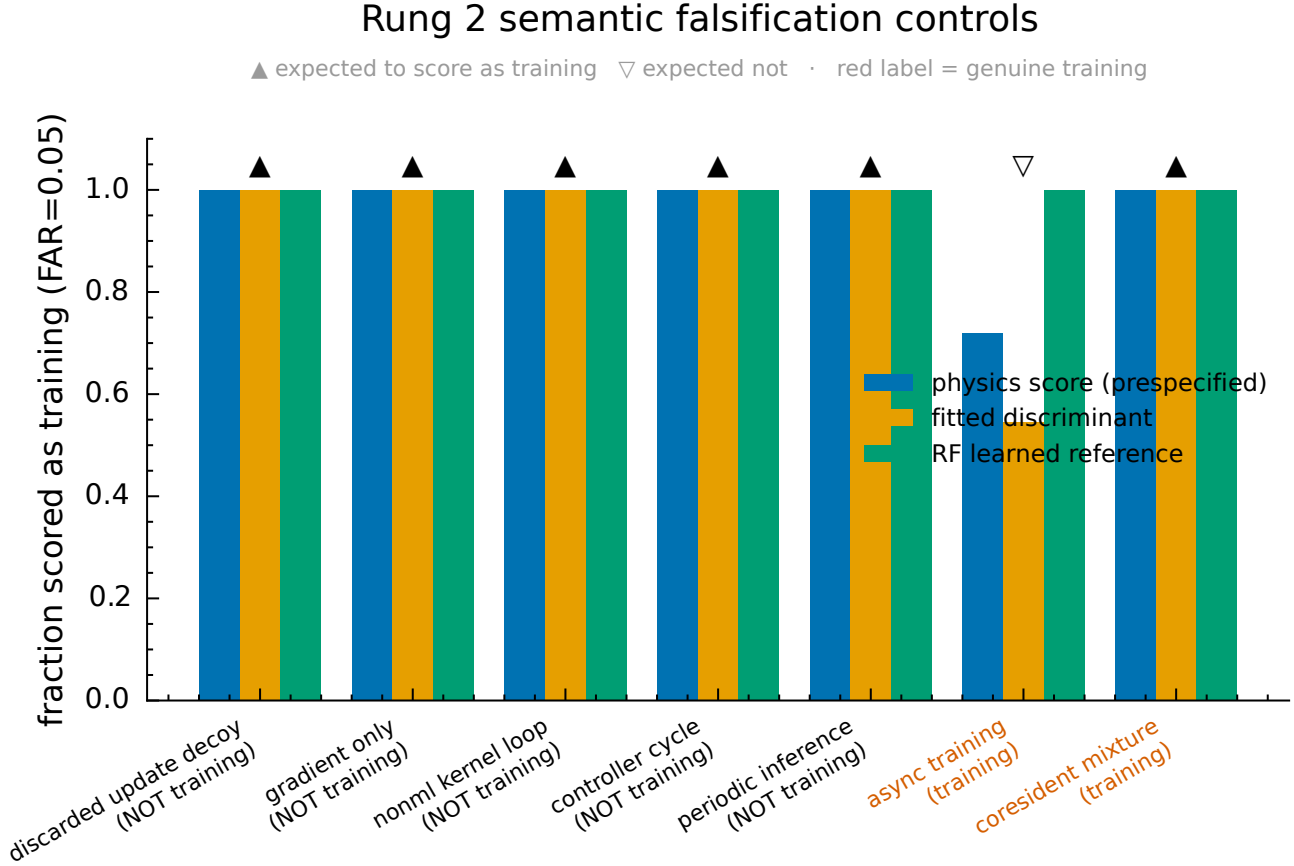
Figure 18. Semantic controls: fraction scored as training per decision rule. The non-training decoys are indistinguishable from training under every rule (the semantic-decoy ceiling); only asynchronous genuine training separates the rules, and the tracked physics rule still catches most of it.
