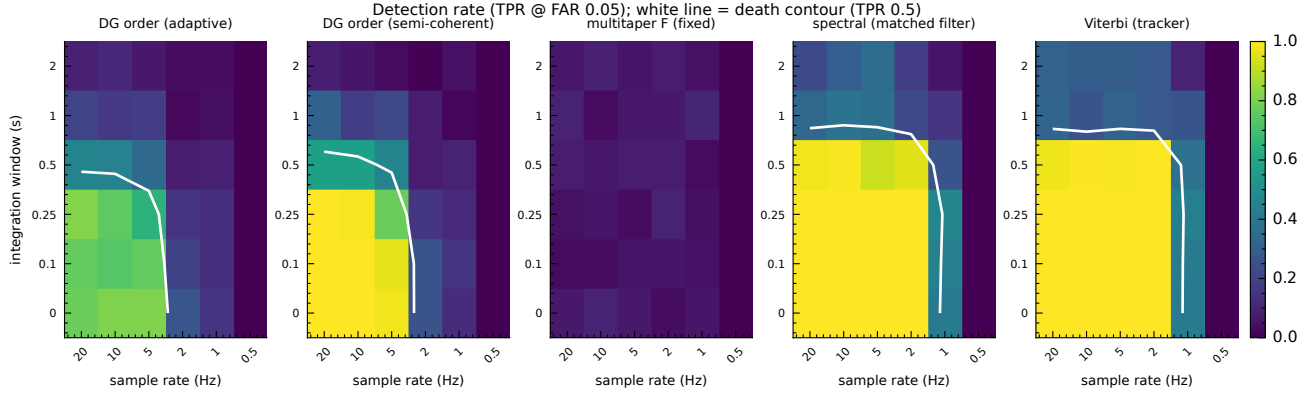
Figure 15. Minimum meter specification: detector power at nominal false-alarm rate 0.05 over sample rate \times integration window, one panel per detector, the honest aggregate against the null aggregate. The live region is sample rate \geq 2 Hz and integration window \leq 0.5 s; below either edge the tracking class collapses toward chance.
