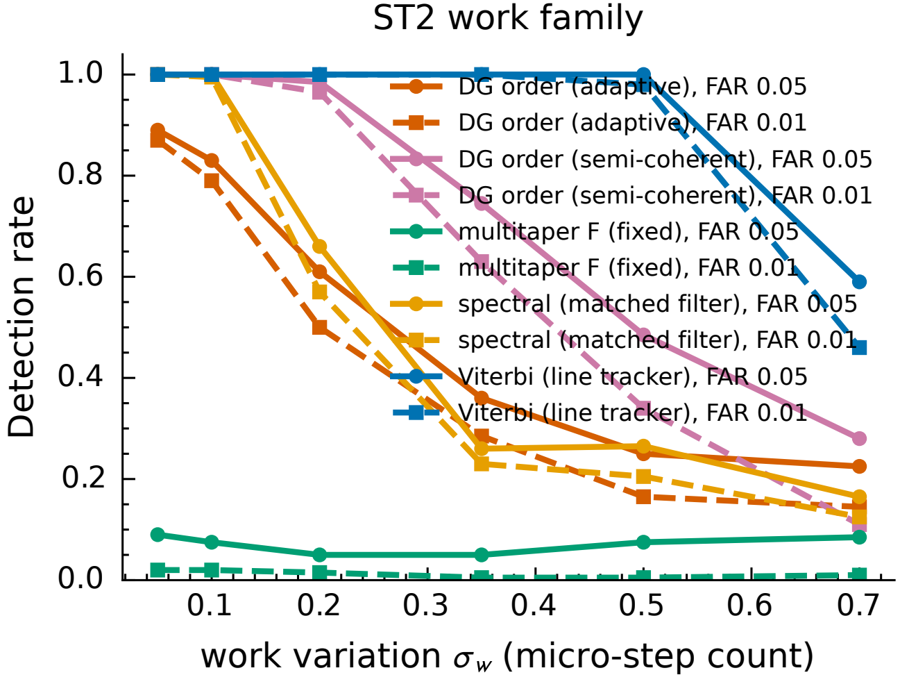
Figure 13. Detector power versus variable-real-work level for each detector. The fixed matched filter and multitaper F-test cross below chance by level 0.35; the tracked order statistics degrade more slowly; the Viterbi tracker holds full power until it finally bends at level 0.7 (detection rate 0.59) — a level whose throughput and learning cost we do not measure.
