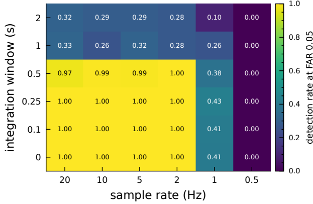
Figure 6. Minimum meter specification: Viterbi detection rate at nominal false-alarm rate 0.05 over sample rate \times integration window, the honest aggregate against the null aggregate ( n = 200 per class). The live region is sample rate \geq 2 Hz and integration window \leq 0.5 s. The per-detector grid is in Appendix E. Reproduced by scripts/plot_st2_meter_boundary.py --scenario aggregate .
