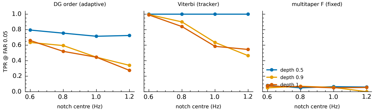
Figure 16. Transfer-function notch sub-sweep at 20 Hz sampling: tracker power versus notch centre frequency and depth. Only a deep notch placed at the cadence centre (1.0–1.2 Hz) materially degrades detection, and it halves rather than erases it.
