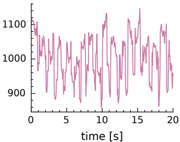
Aggregate, dominant share 0.5
