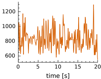
Null aggregate, dominant share 0.5
