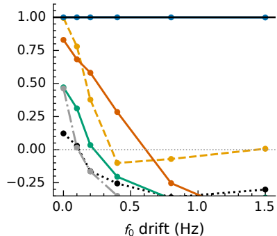
fraction of NP-optimal power (vs inference null)
