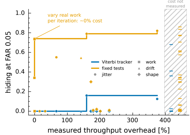
Figure 6. Cost of hiding. Measured throughput overhead against hiding (1– detection rate at false-alarm rate 0.05) for the four adversarial strategies with a hardware cost anchor, with the Pareto staircase — the best hiding available at or below a given cost — against the fixed tests (orange; the better of the matched filter and multitaper F-test per cell) and the Viterbi tracker (blue). Varying real work per iteration hides \sim 0.74 from the fixed tests at no measurable cost; against the tracker no anchored attack hides more than 0.16. Cells without a cost anchor are shown as ticks in the hatched strip, among them work-variation level 0.7, where the tracker begins to fail. Reproduced by scripts/plot_money_pareto.py .
