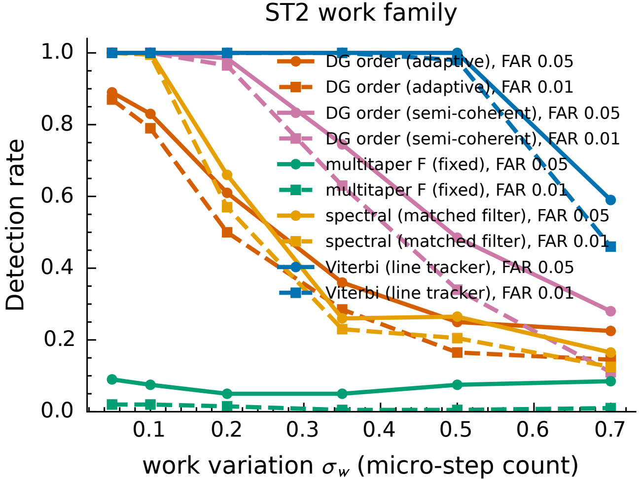
Figure 11. Detector power versus variable-real-work level for each detector. The fixed matched filter and multitaper F-test cross below chance by level 0.35; the tracked order statistics degrade more slowly; the Viterbi tracker holds full power until it finally bends at level 0.7 (detection rate 0.59) — a level whose throughput and learning cost we do not measure.
