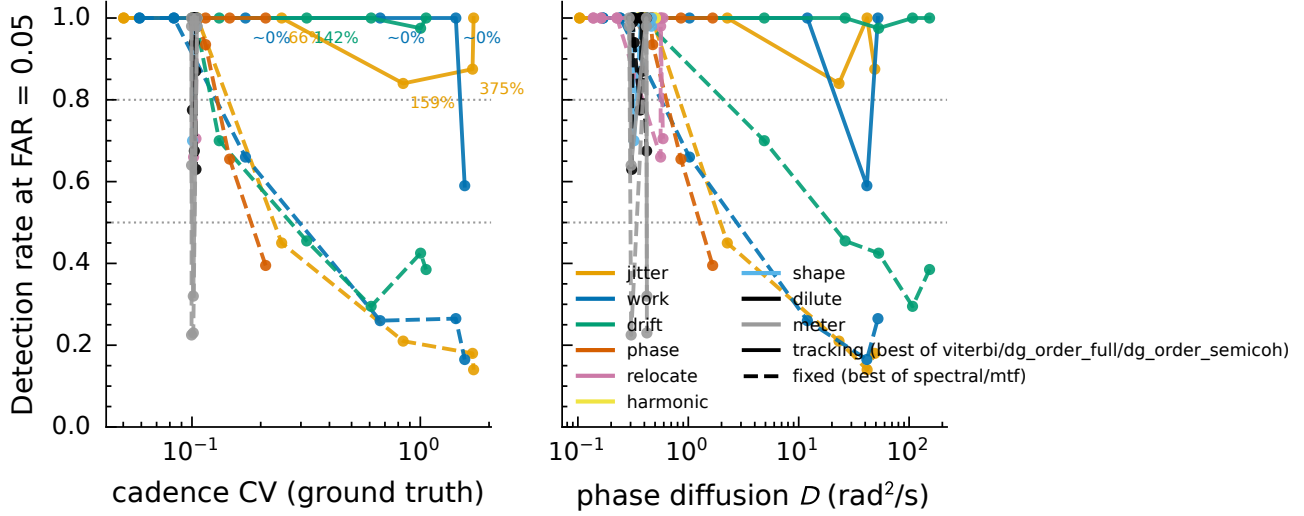
Figure 10. The de-periodicisation frontier: physical de-periodicisation (cadence coefficient of variation) against best tracking and best fixed detector power at nominal false-alarm rate 0.05, over all adversarial strategies. The near-vertical drop of the fixed class at the variable-real-work strategy, at essentially zero throughput cost, while the tracking class holds, is the scope boundary; costlier strategies (idle jitter, drift, shaping) sit at high throughput overhead without erasing the tracked line.
