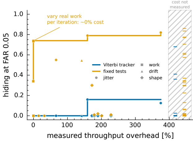
Figure 7. Cost of hiding. Measured throughput overhead against hiding (1— detection rate at false-alarm rate 0.05) for the four adversarial strategies with a hardware cost anchor, with the Pareto staircase — the best hiding available at or below a given cost — against the fixed tests (orange; the better of the matched filter and multitaper F-test per cell) and the Viterbi tracker (blue). Varying real work per iteration hides \sim 0.74 from the fixed tests at no measurable cost; against the tracker no anchored attack hides more than 0.16. Cells without a cost anchor are shown as ticks in the hatched strip, among them work-variation level 0.7, where the tracker begins to fail. Reproduced by scripts/plot_money_pareto.py .
