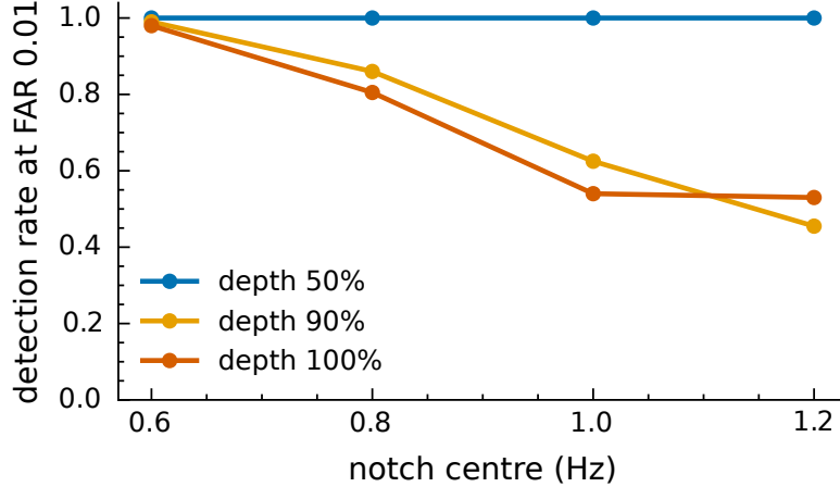
Figure 9. Notch sweep: Viterbi detection rate at empirical false-alarm rate 10^{-2} versus notch centre, one line per notch depth, at 20 Hz sampling with no integration window, the honest aggregate against the null aggregate ( n = 200 per class). A deep notch near the band centre roughly halves detection; none removes it.
