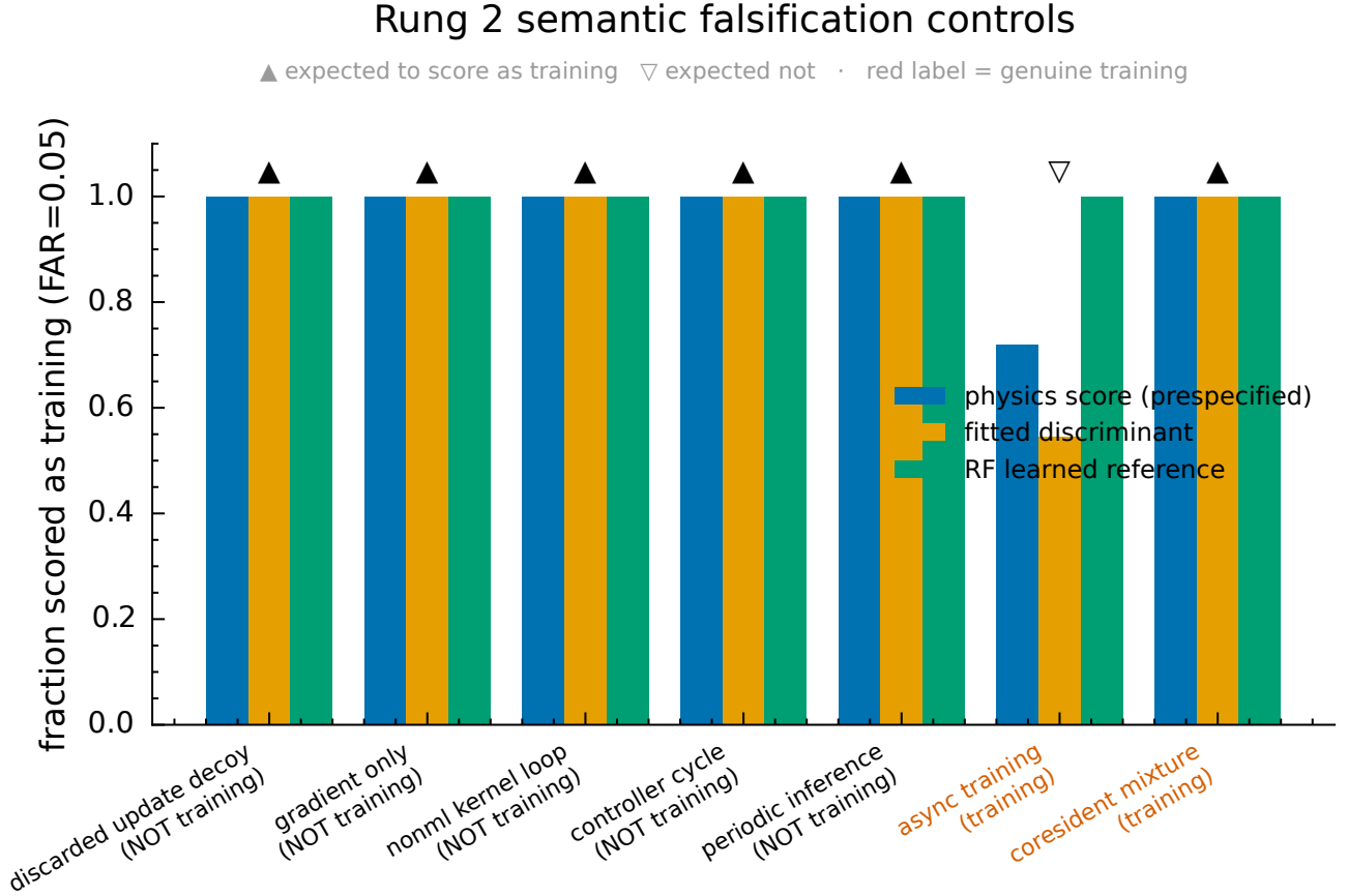
Figure 17. Semantic controls: fraction scored as training per decision rule. The non-training decoys are indistinguishable from training under every rule (the semantic-decoy ceiling); only asynchronous genuine training separates the rules, and the tracked physics rule still catches most of it.
