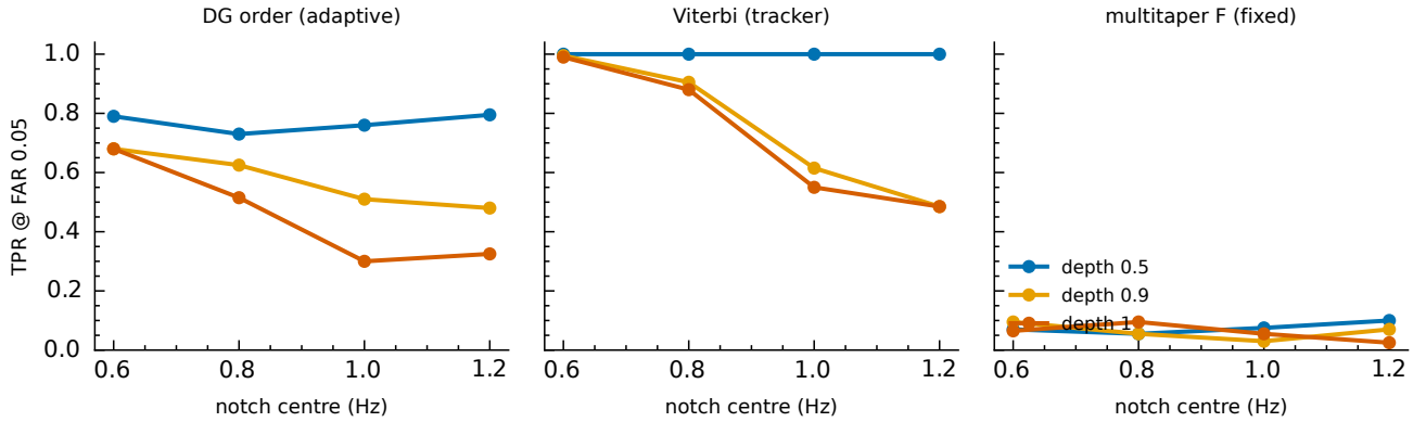
Figure 15. Transfer-function notch sub-sweep at 20 Hz sampling: tracker power versus notch centre frequency and depth. Only a deep notch placed at the cadence centre (1.0–1.2 Hz) materially degrades detection, and it halves rather than erases it.
