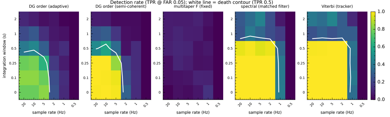
Figure 14. Minimum meter specification: detector power at nominal false-alarm rate 0.05 over sample rate \times integration window, one panel per detector, honest training against the hard inference null. The live region is sample rate \geq 2 Hz and integration window \leq 0.5 s; below either edge the tracking class collapses toward chance.
