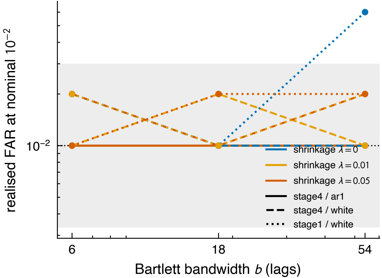
Figure 5. The covariance-estimator sweep is the fix-or-reframe axis: realised rate at nominal 10^{-2} versus Bartlett bandwidth b for each shrinkage. The bandwidth that repairs the fully adaptive stage (stage 4) inflates the fixed- \alpha anchor (stage 1). No single configuration calibrates both.
