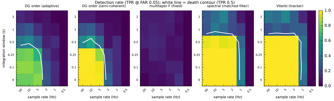
Figure 3. Minimum meter specification: detector power at nominal false-alarm rate 0.05 over sample rate \times integration window, one panel per detector, honest training against the hard inference null. The live region is sample rate \geq 2 Hz and integration window \leq 0.5 s; below either edge the tracking class collapses toward chance.
