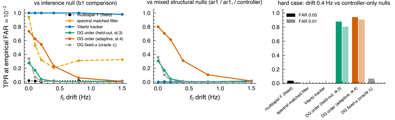
Figure 6. Detector bake-off on the cadence-drift axis: detection rate at empirical false-alarm rate versus drift, for each detector and both negative classes. Only the tracked order family retains power against the structural negatives; the spectral-shape detectors detect the controller third of the mix more strongly than the signal.
