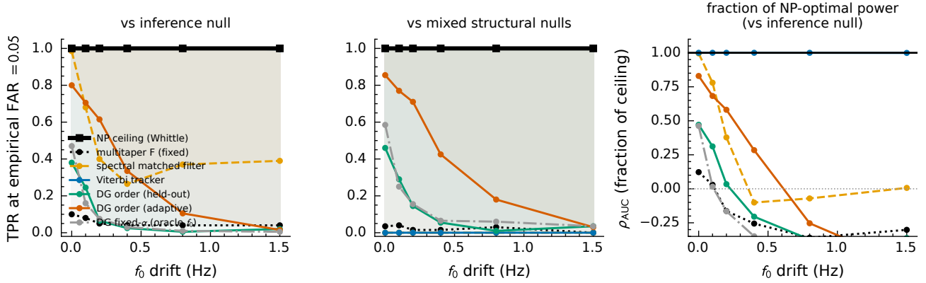
Figure 7. Corpus-free detectors as a fraction of the Whittle Neyman–Pearson ceiling versus cadence drift, against the inference null and the structural confusers. The ceiling is 1.0 everywhere; the Viterbi tracker saturates it against the inference null, while only the tracked order family approaches it against the structural confusers. The gap that opens at high drift is the headroom above current detectors.
