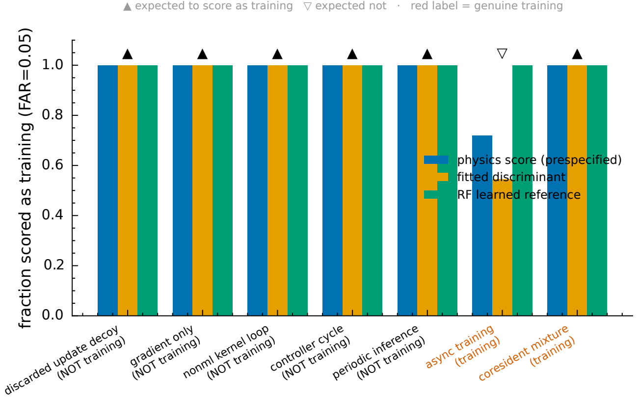
Figure 18. Semantic controls: fraction scored as training per decision rule. The non-training decoys are indistinguishable from training under every rule (the semantic-decoy ceiling); only asynchronous genuine training separates the rules, and the tracked physics rule still catches most of it.
