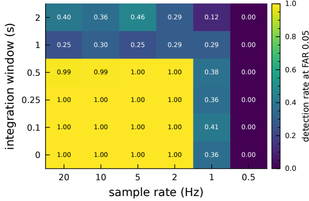
Figure 6. Minimum meter specification: Viterbi detection rate at nominal false-alarm rate 0.05 over sample rate \times integration window, honest training against the inference null ( n = 200 per class). The live region is sample rate \geq 2 Hz and integration window \leq 0.5 s. The per-detector grid is in Appendix E. Reproduced by scripts/plot_st2_meter_boundary.py .
