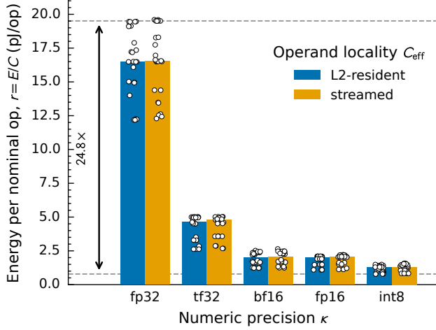
Figure 3. The exchange-rate band of Equation (22) (Experiment 1). Total energy quotient E/C for a fixed matmul kernel on an NVIDIA A100, swept factorially over precision \kappa , operand locality C_{\text{eff}} (paired bars), and operand distribution \alpha ; white points are the individual measured windows ( n = 240 across 60 cells). Dashed lines mark the band edges: the dearest cell is the band ceiling r_{\text{hi}} , the cheapest (int8, zero operands) the envelope floor r_{\text{lo}} .
