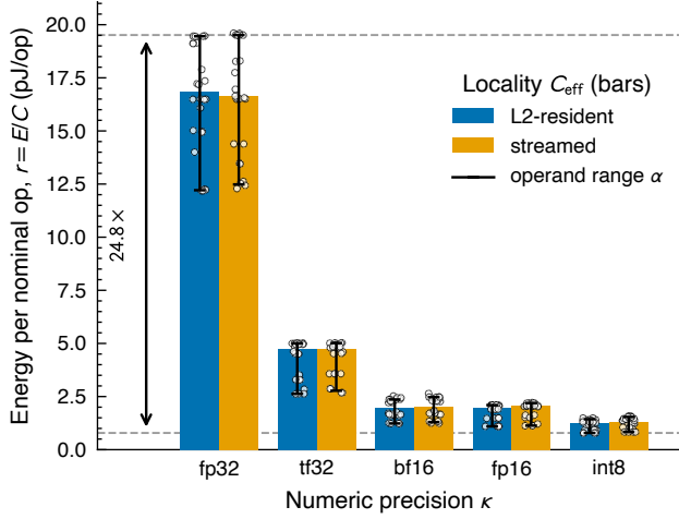
Figure 3. The exchange-rate band of Equation (22) (Experiment 1). Total energy quotient E/C for a fixed matmul kernel on an NVIDIA A100, swept factorially over precision \kappa (bar groups), operand locality C_{\text{eff}} (paired bars), and operand distribution \alpha (whiskers); white points are the individual measured windows ( n = 240 across 60 cells). Each bar is the median over the operand axis and its whisker that axis’s full range, so the operand factor—a little under 2\times inside every format, against locality’s couple of percent—is read off the figure rather than pooled into it. Dashed lines mark the band edges, both of them operand extremes: the ceiling r_{\text{hi}} is fp32 at its dearest operands, the floor r_{\text{lo}} int8 with zeros.
