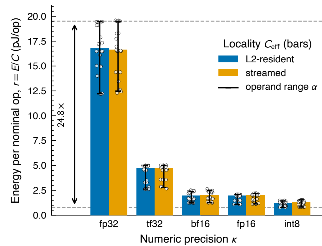
Figure 3. The measured energy quotient E/C , swept factorially over precision (bar groups), locality (paired bars) and operand distribution (whiskers); dashed lines mark the band edges.
