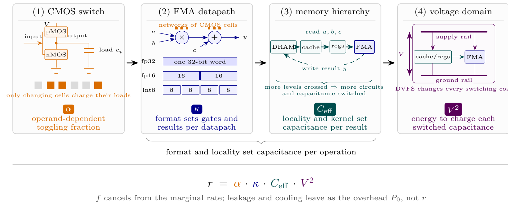
Figure 2. The exchange rate assembled across physical scales, from a single CMOS switch to the powered die.
