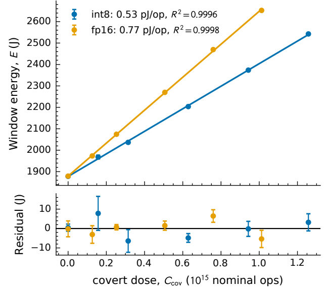
Figure 6. The marginal covert cost (Experiment 7): window energy E vs. covert dose C_{\text{cov}} for int8 and fp16 covert work, added to a fixed fp16 declared burst inside a fixed 10 s window. Top : per-cell medians with \pm 1 SD error bars over the five repeats, against the dose fit E = r_{\text{cov}} C_{\text{cov}} + E_0 ; both slopes are linear to R^2 > 0.999 (0.53 pJ/op int8, 0.77 pJ/op fp16) and share a zero-dose intercept matching the directly measured zero-dose windows to 0.02%. Bottom : residuals. Because the baseline burns identically at every dose, it cancels in the slope: unlike the between-shape fit of Figure 5, this within-cell slope is the incremental estimand \partial E / \partial C_{\text{cov}} the floor’s covert denominator requires (Theorem 4.1).
