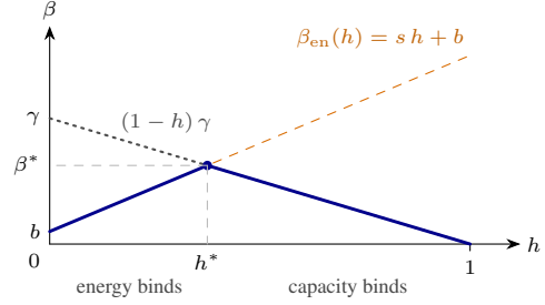
Figure 3. The shape of the floor. The energy-only width \beta_{\text{en}}(h) = sh + b rises with declared utilisation—more honest work offers more cover (dashed)—while the capacity clip (1-h)\gamma falls, since more honest work leaves less machine free (dotted). The floor Equation (21) is the lower of the two (solid): a tent peaking at the crossing (h^*, \beta^*) of Equation (22), with energy binding to its left, capacity to its right, and \beta(1) = 0 because a fully occupied machine leaves nowhere to hide. No numeric scale is intended—the s, b and \gamma drawn here are illustrative, and Figure 8 plots the same construction on measured bands.
