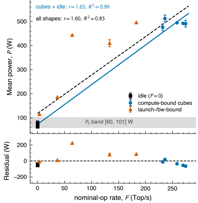
Figure 5. The overhead band and the affine forward map (Experiment 3, n = 65 windows across a 15-cell rate ladder). Top : mean power P vs. nominal-op rate F , plotted as per-cell medians with \pm 1 SD error bars over each cell’s repeats. Markers give each cell’s shape class: idle anchors (black, F = 0 ), compute-bound cubes ( M = N = K \geq 2048 , blue), and the launch- and bandwidth-bound mid-ladder shapes (orange). Two affine fits P = rF + P_0 are overlaid: the like-for-like fit over the idle anchors and the cubes alone (blue, r = 1.65 pJ/op, R^2 = 0.99 ), and the pooled fit over all fifteen cells (black dashed, r = 1.60 pJ/op, R^2 = 0.852 ). The slope moves by 4% between them while the scatter grows sharply, so the off-class shapes account for the residual and not for the rate. The shaded band is the observed idle range across five idle variants, P_0 \in [59.8, 101.0] W, read directly off those cells rather than from either fitted intercept. Bottom : residuals about the pooled fit, which is what its R^2 measures; the orange shapes carry the scatter. This is a between-shape diagnostic of the affine map; the covert denominator the floor actually uses is the within-cell marginal cost of Figure 6 (Experiment 4), not either fit here.
