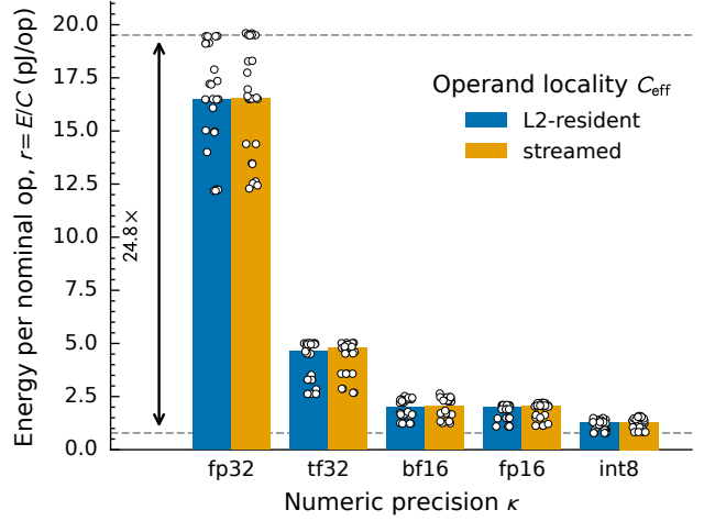
Figure 3. The exchange-rate band of Equation (21) (Experiment 1). Total energy quotient E/C for a fixed matmul kernel on an NVIDIA A100, swept factorially over precision \kappa , operand locality C_{eff} (paired bars), and operand distribution \alpha ; white points are the individual measured windows ( n = 240 across 60 cells). Dashed lines mark the band edges: the dearest cell is the band ceiling r_{hi} , the cheapest (int8, zero operands) the envelope floor r_{lo} .
