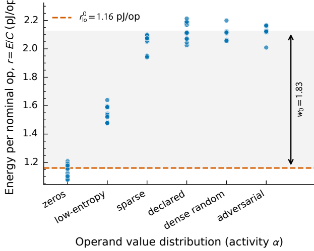
Figure 4. The operand envelope (Experiment 2, n = 96 windows across six operand distributions). Kernel, shape, and precision (fp16) are held fixed and only the operand values vary; the SM clock was governor-selected, not locked, so the families do not share a common clock stratum (Section 5.3). The figure is a descriptive within-device map of how far operand activity alone stretches r , not a clean isolation of the activity factor \alpha . The shaded span is the observed operand spread w_0 = 1.83 ; the minimum (zeros, dashed) is the descriptive fp16 operand floor r_{lo}^0 = 1.16 pJ/op as a total quotient. That floor is not the covert denominator: r_{lo}^{cov} is Experiment 4’s marginal edge. Like for like, the fp16 marginal edge is 0.76 pJ/op—cheaper than this quotient by the baseline power the quotient amortises; the headline 0.51 is cheaper again because it is int8.
