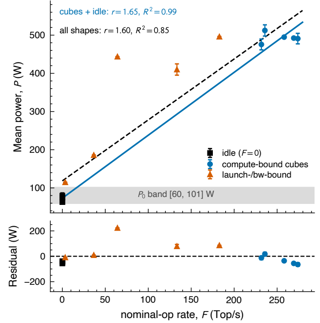
Figure 6. The overhead band and the affine forward map (Experiment 2, n = 65 windows across a 15-cell rate ladder). Top : mean power P vs. nominal-op rate F , plotted as per-cell medians with \pm 1 SD error bars over each cell’s repeats. Markers give each cell’s shape class: idle anchors (black, F = 0 ), compute-bound cubes ( M = N = K \geq 2048 , blue), and the launch- and bandwidth-bound mid-ladder shapes (orange). Two affine fits P = rF + P_0 are overlaid: the like-for-like fit over the idle anchors and the cubes alone (blue, r = 1.65 pJ/op, R^2 = 0.99 ), and the pooled fit over all fifteen cells (black dashed, r = 1.60 pJ/op, R^2 = 0.852 ). The slope moves by 4% between them while the scatter grows sharply, so the off-class shapes account for the residual and not for the rate. The shaded band is the observed idle range across five idle variants, P_0 \in [59.8, 101.0] W, read directly off those cells rather than from either fitted intercept. Bottom : residuals about the pooled fit, which is what its R^2 measures; the orange shapes carry the scatter. This is a between-shape diagnostic of the affine map; the covert denominator the floor actually uses is the within-cell marginal cost of Figure 7 (Experiment 3), not either fit here.
