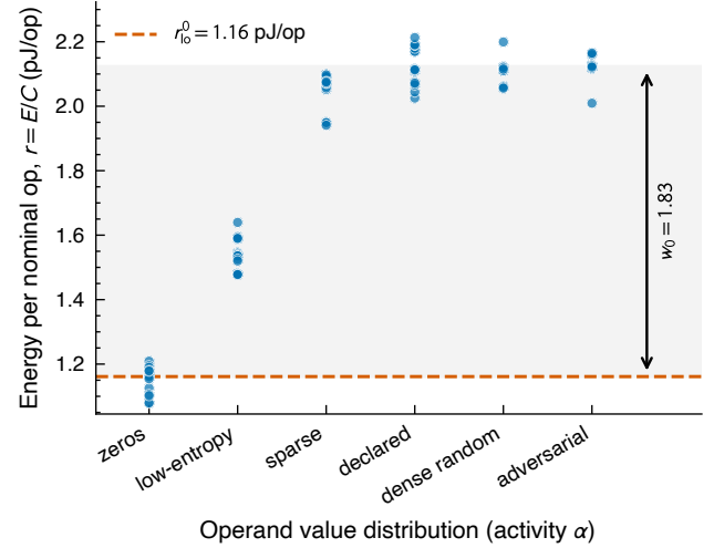
Figure 6. The operand envelope (Experiment 2, n = 96 windows across six operand distributions). Kernel, shape, and precision (fp16) are held fixed and only the operand values vary; the clock was governor-selected, not locked, so the map is descriptive (see text). The shaded span is the observed operand spread w_0 = 1.83 ; the minimum (zeros, dashed) is the descriptive fp16 operand floor r_{\text{lo}}^0 = 1.16 pJ/op as a total quotient—not the covert denominator, which is Experiment 4’s marginal edge.
