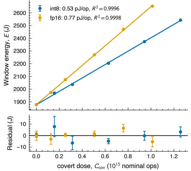
Figure 8. The marginal covert cost (Experiment 4): window energy E vs. covert dose C_{\text{cov}} for int8 and fp16 covert work, added to a fixed fp16 declared burst inside a fixed 10 s window. Top : per-cell medians with \pm 1 SD error bars over each cell’s four untrimmed repeats (of five captured; the flagged high-tail repeat is excluded), against the dose fit E = r_{\text{cov}} C_{\text{cov}} + E_0 ; both slopes are linear to R^2 > 0.999 (0.53 pJ/op int8, 0.77 pJ/op fp16) and share a zero-dose intercept matching the directly measured zero-dose windows to 0.02%. Bottom : residuals. Because the baseline burns identically at every dose, it cancels in the slope: unlike the between-shape fit of Figure 7, this within-cell slope is the incremental estimand \partial E / \partial C_{\text{cov}} the floor’s covert denominator requires (Appendix C).
