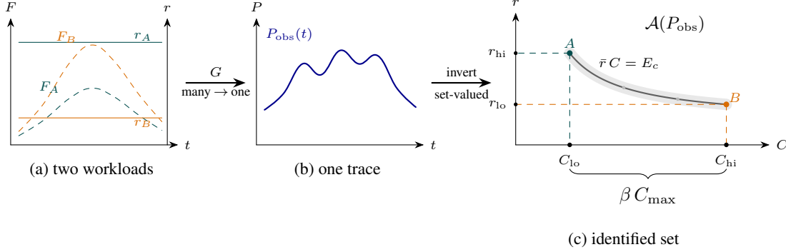
Figure 1. Non-injectivity of the forward map. (a) Two workloads ( A little compute at a high rate, B much compute at a low rate) whose products rF coincide, so (b) they drive the identical power trace. (c) Inverting recovers only the set of consistent explanations \mathcal{A}(P_{\text{obs}}) : the rate band [r_{\text{lo}}, r_{\text{hi}}] cuts the constant-energy arc A-B , whose projection onto the C -axis spans [C_{\text{lo}}, C_{\text{hi}}] ; relative to capacity that width is the floor \beta . The faint ribbon is meter noise (ignored in this work). Each rate is drawn constant only for clarity; in reality r(t) varies in time. This does not matter for a question about total operations, which depends on r(t) only through its op-weighted mean \bar{r} = E_c/C (compute energy E_c = \int_0^T rF dt over total operations C ). That mean is panel (c)'s vertical axis, so letting r(t) vary leaves the picture unchanged.
