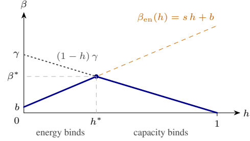
Figure 3. The shape of the floor. The energy-only width \beta_{\text{en}}(h) = s h + b rises with declared utilisation—more honest work offers more cover (dashed)—while the capacity clip (1-h)\gamma falls, since more honest work leaves less machine free (dotted). The floor Equation (21) is the lower of the two (solid): a tent peaking at the crossing (h^*, \beta^*) of Equation (23), with energy binding to its left, capacity to its right, and \beta(1) = 0 because a fully occupied machine leaves nowhere to hide. No numeric scale is intended—the s , b and \gamma drawn here are illustrative, and Figure 8 plots the same construction on measured bands.
