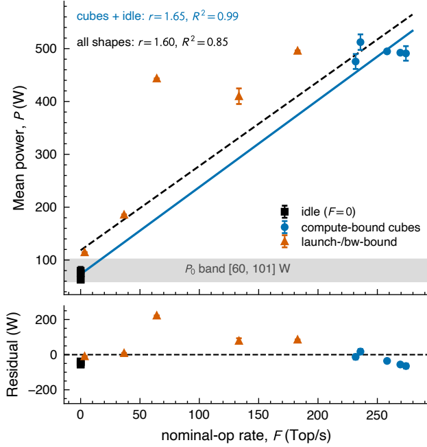
Figure 6. The overhead band and the affine forward map (Experiment 2, n = 65 windows across a 15-cell rate ladder). Top : mean power P vs. nominal-op rate F , plotted as per-cell medians with \pm 1 SD error bars over each cell’s repeats. Markers give each cell’s shape class: idle anchors (black, F = 0 ), compute-bound cubes ( M = N = K \geq 2048 , blue), and the launch- and bandwidth-bound mid-ladder shapes (orange). Two affine fits P = rF + P_0 are overlaid: the like-for-like fit over the idle anchors and the cubes alone (blue, r = 1.65 pJ/op, R^2 = 0.99 ), and the pooled fit over all fifteen cells (black dashed, r = 1.60 pJ/op, R^2 = 0.852 ). The slope moves by 4% between them while the scatter grows sharply, so the off-class shapes account for the residual and not for the rate. The shaded band is the observed idle range across five idle variants, P_0 \in [59.8, 101.0] W, read directly off those cells rather than from either fitted intercept. Bottom : residuals about the pooled fit, which is what its R^2 measures; the orange shapes carry the scatter. This is a between-shape diagnostic of the affine map; the covert denominator the floor actually uses is the within-cell marginal cost of Figure 7 (Experiment 3), not either fit here.
