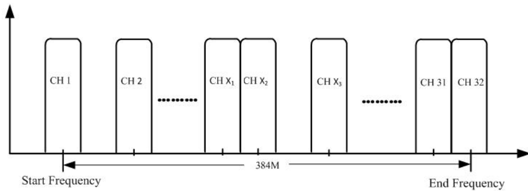
Carrier Setting Illustration:
