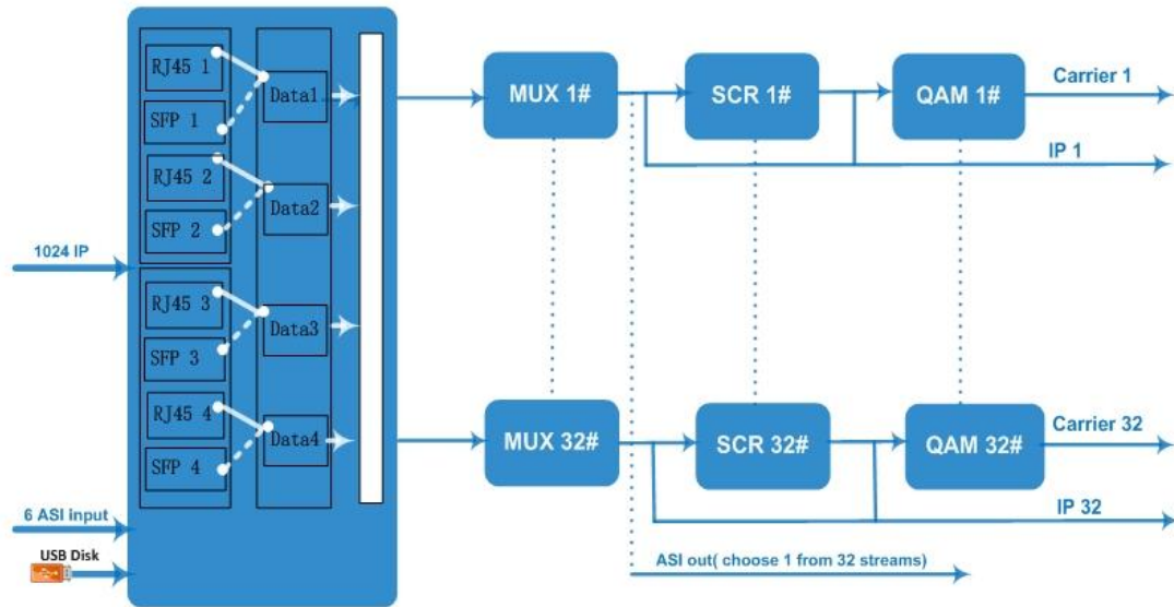
Carrier Setting Illustration:
