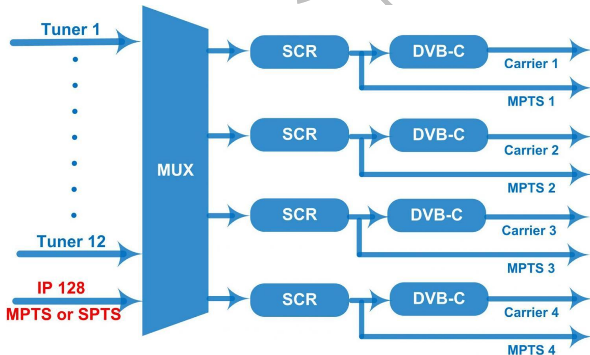
FU-4459CS DVB-C Principle Chart
