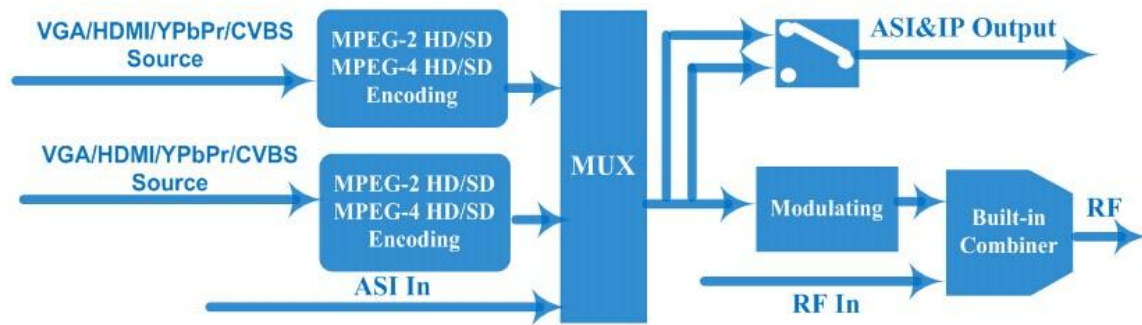
Principle Chart(Modulator)
