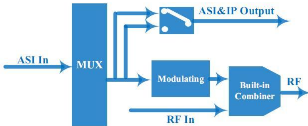
Principle Chart(Modulator)
