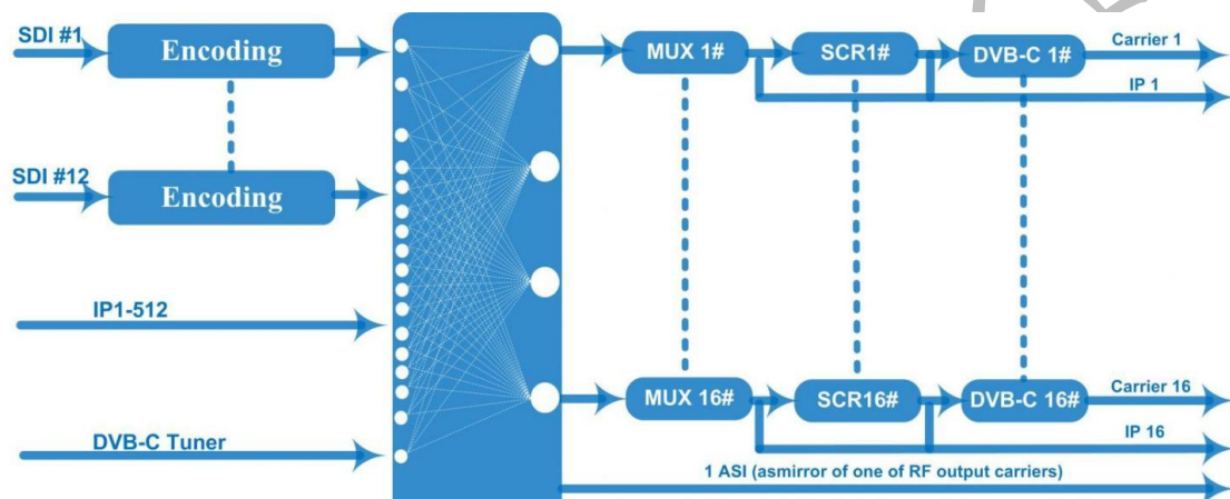
DVB-C Principle Chart
