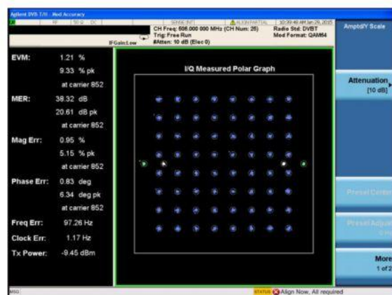
Figure 6 MER (64 QAM)
