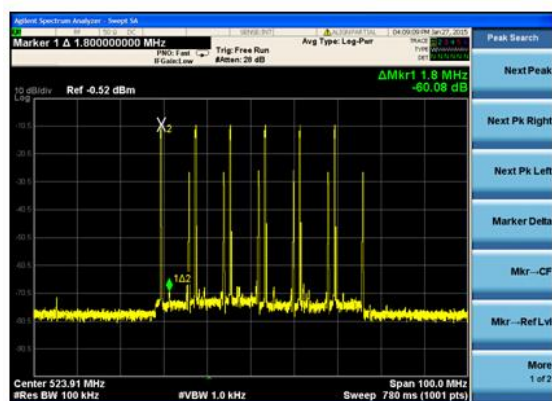
Figure 9 In-band Spurious
