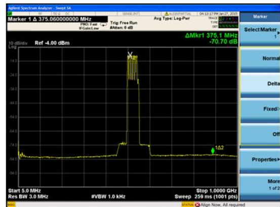
Figure 8 Out-band Rejection
