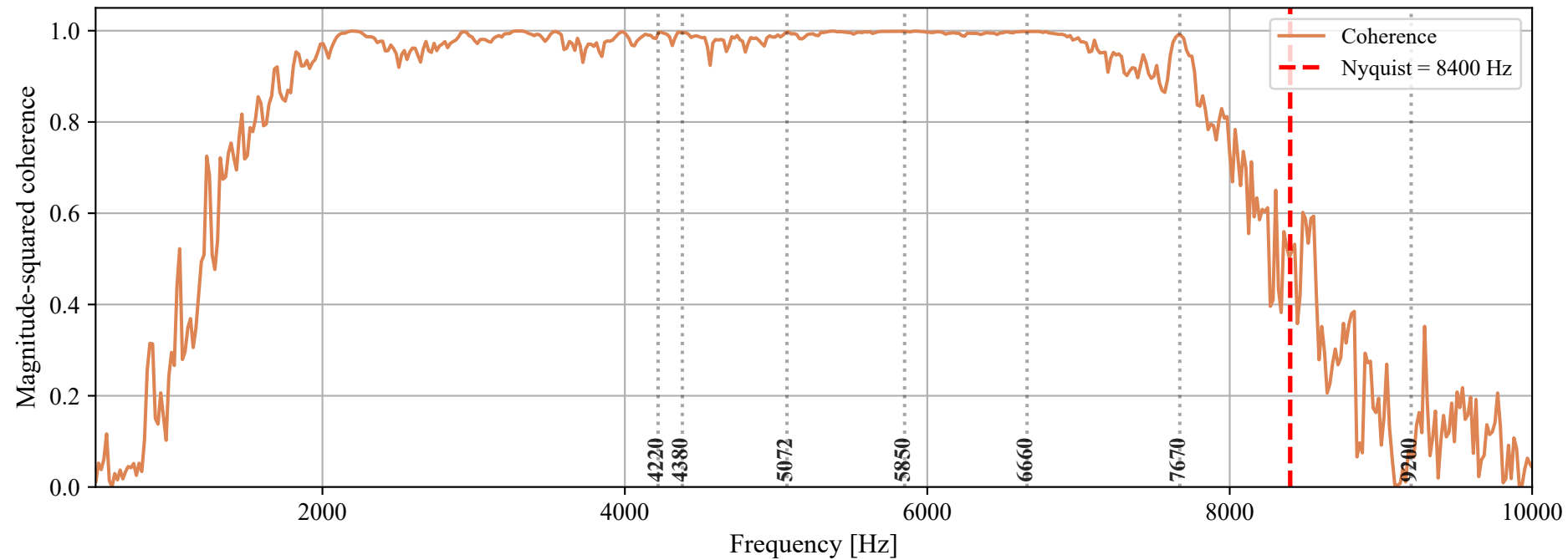
Coherence between true disturbance and MMP from DOB estimate
