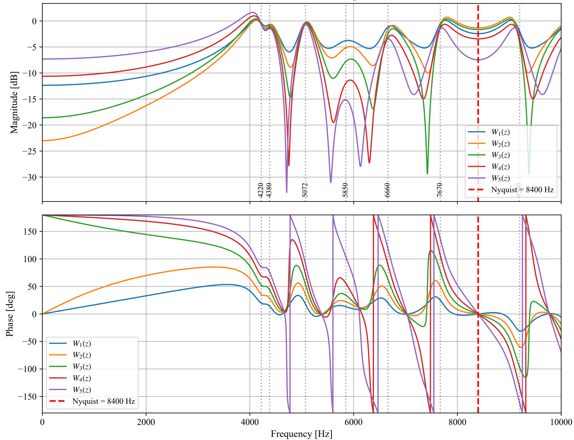
IIR-MMP Bode response, L=6 , a_g=0.94
