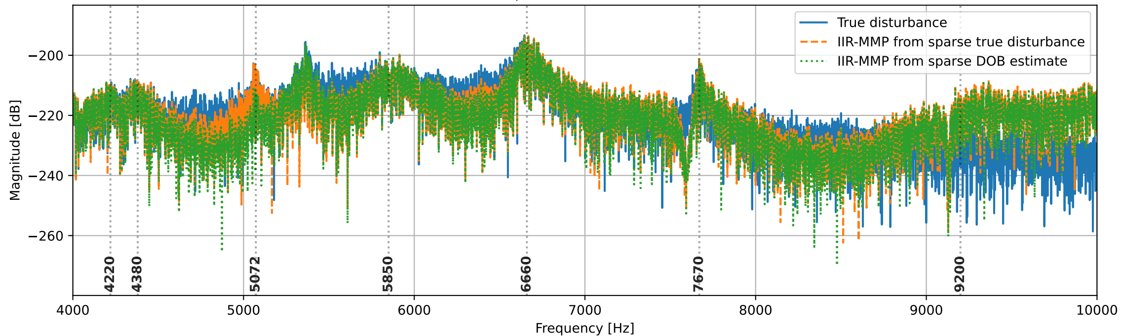
FFT comparison, disturbance band
