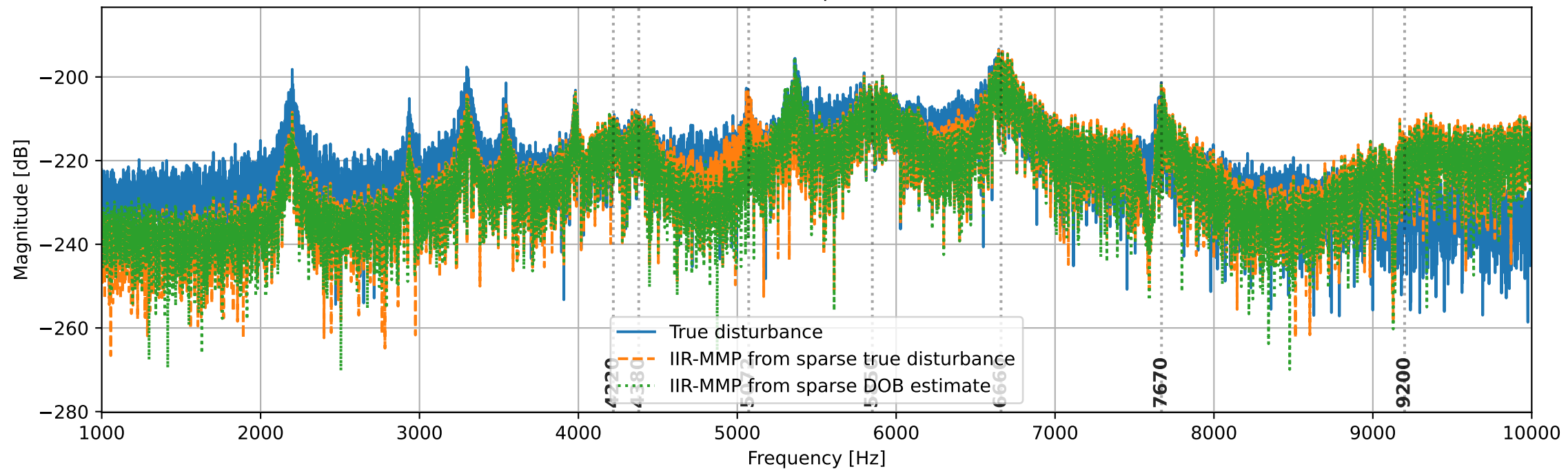
FFT comparison
