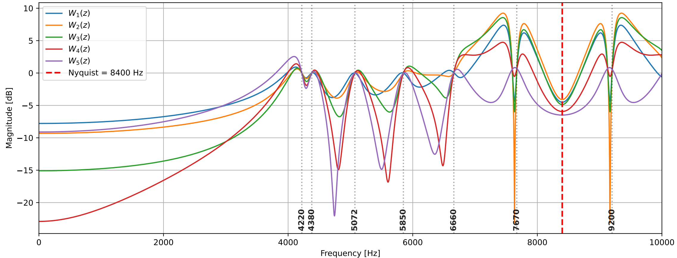
IIR-MMP Bode magnitude, L=6 , a_g=0.94
