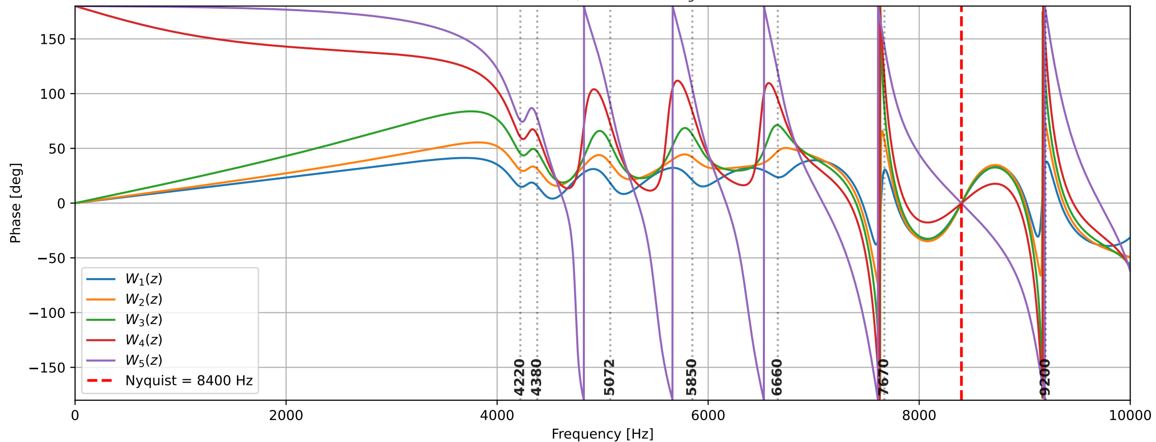
IIR-MMP Bode phase, L=6 , a_g=0.94
