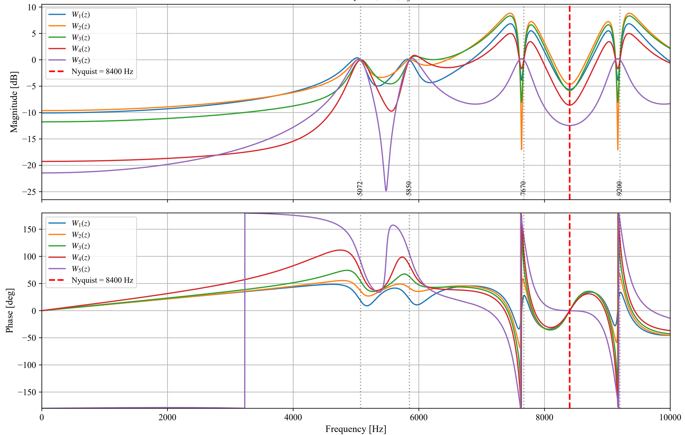
IIR-MMP Bode response, L=6 , a_g=0.94
