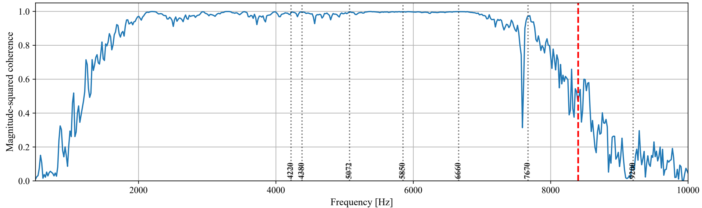
Coherence between true disturbance and MMP from DOB estimate
