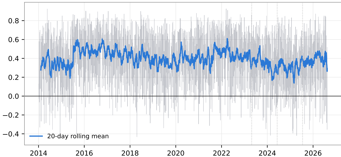
Daily rank IC of incremental signal
