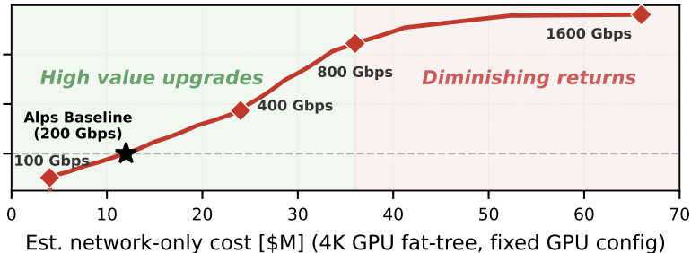
Relative Performance vs Alps Baseline
