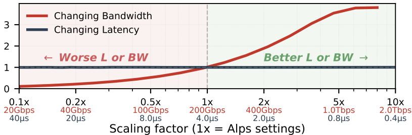
Relative Performance vs Alps Baseline
