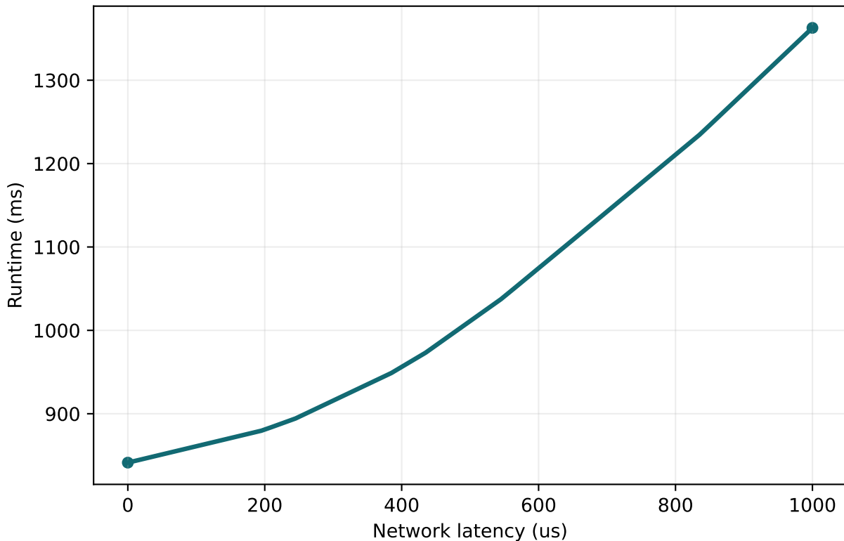
Fig. 5 Llama7B Composite-LP historical mode Regenerated
