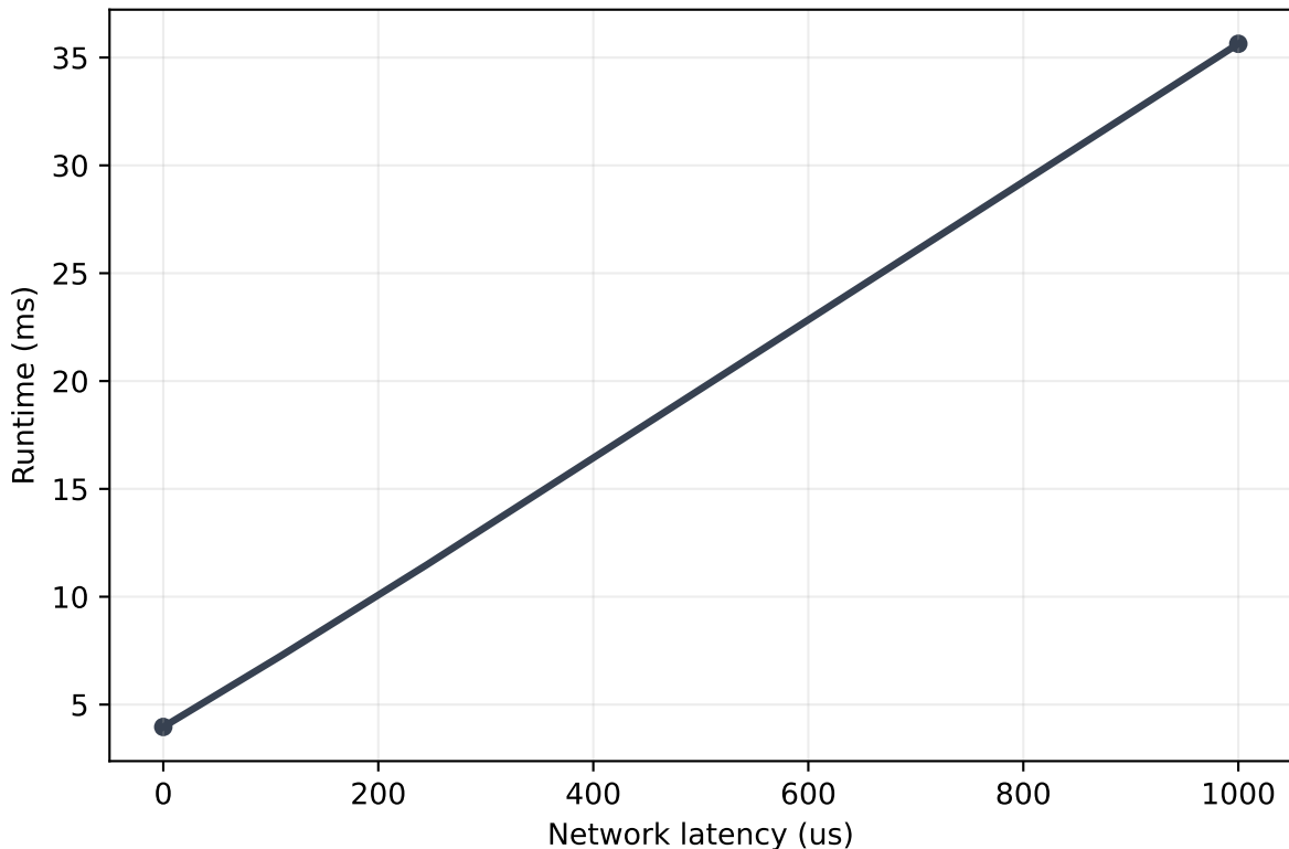
Fig. 3 AllReduce 128MiB, 16 nodes, auto channels Paper/reference
